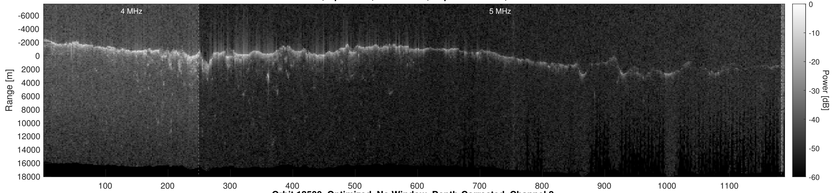
Orbit 12500, Optimized, No Window, Depth-Corrected, Channel 2
