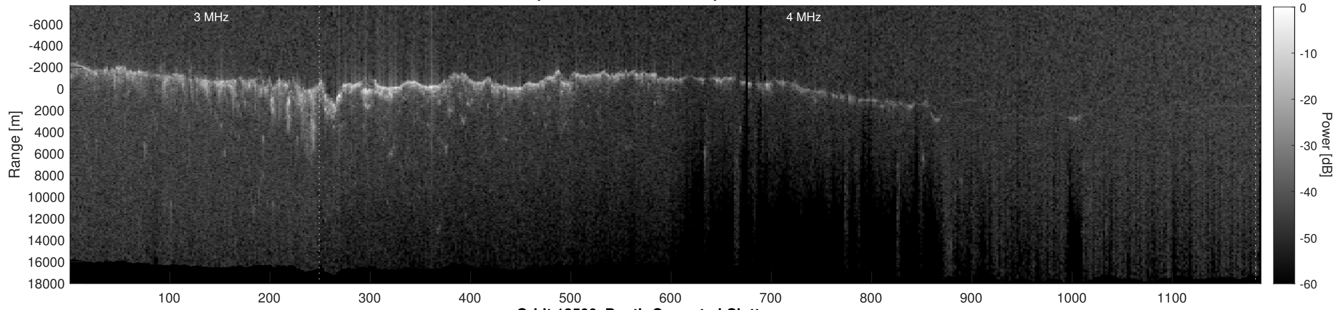
Orbit 12500, Depth-Corrected Cluttergram
