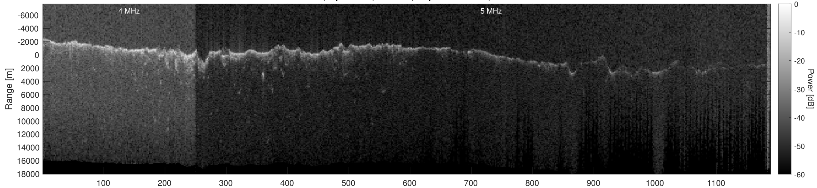
Orbit 12500, Optimized, Window, Depth-Corrected, Channel 2
