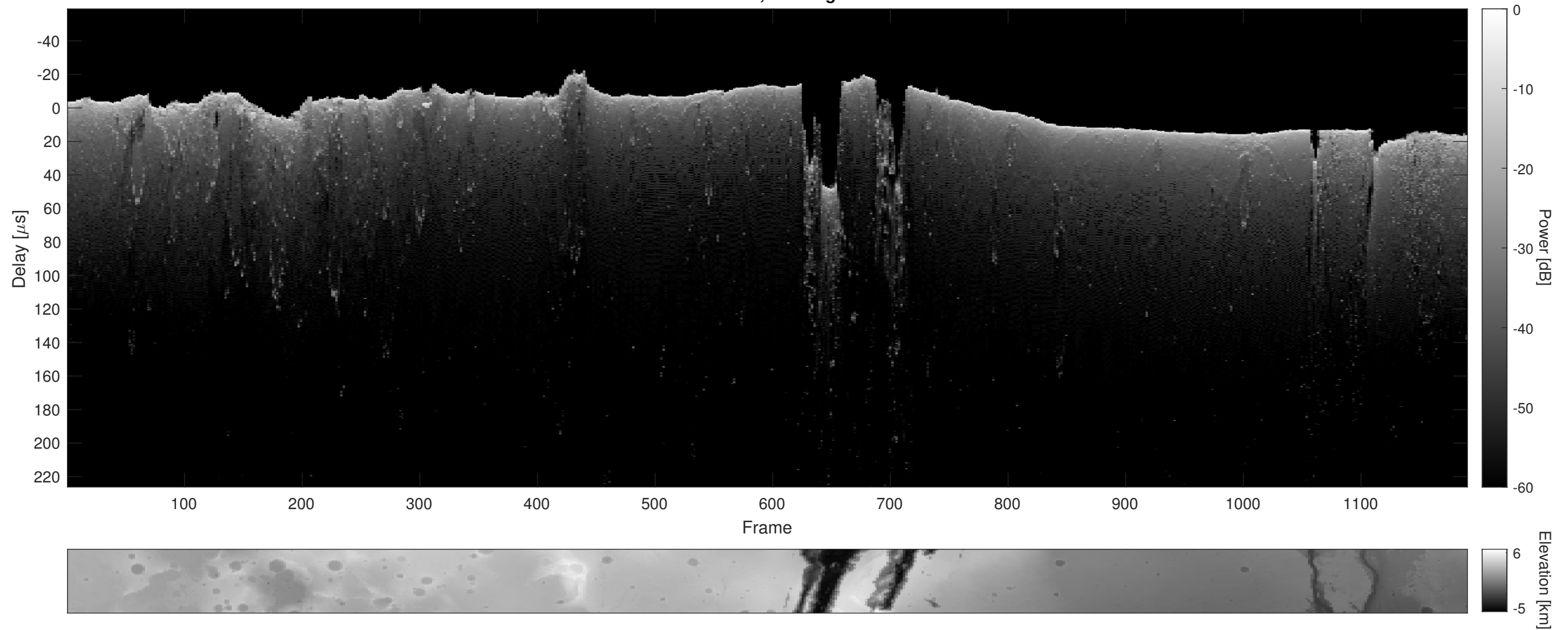
Orbit 12501, Cluttergram
