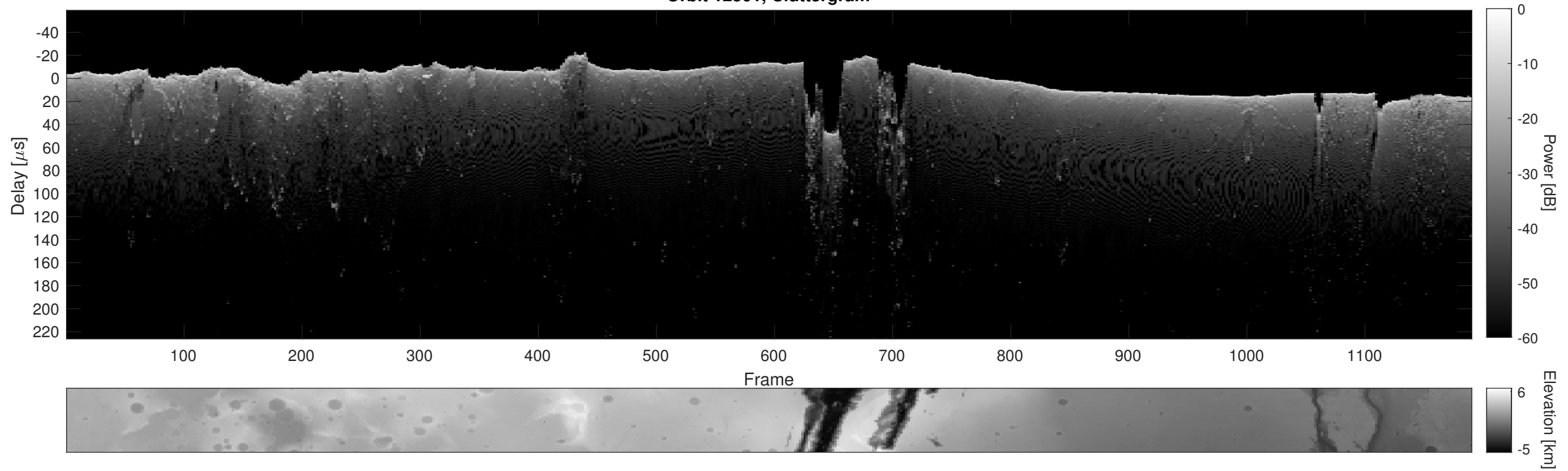
Orbit 12501, Cluttergram
