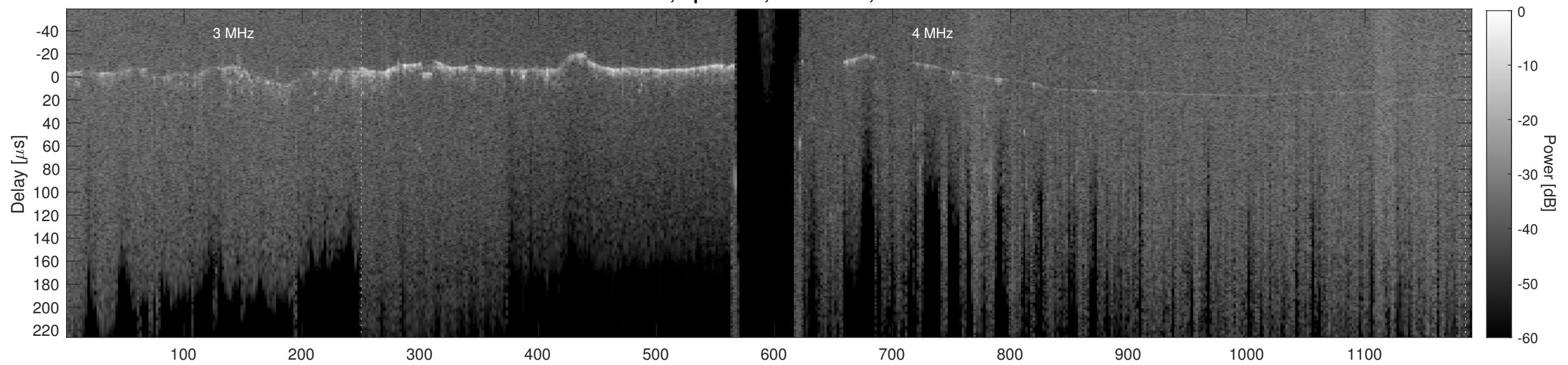
Orbit 12501, Cluttergram
