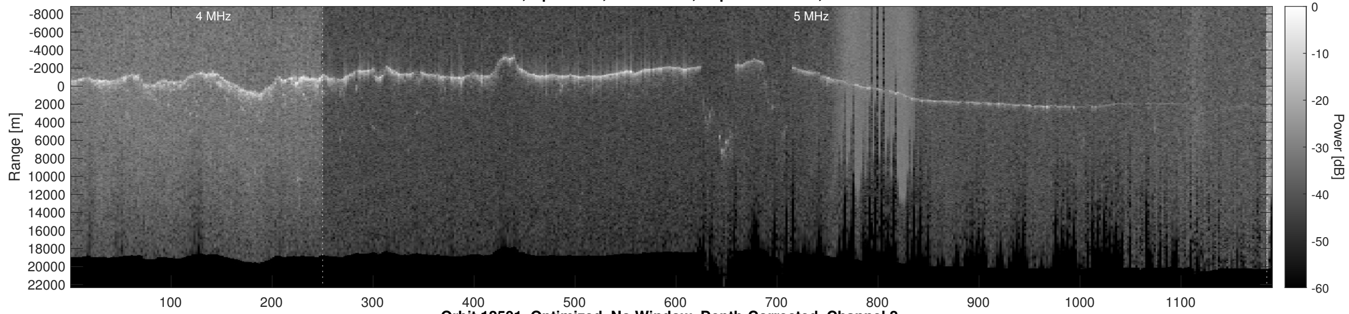
Orbit 12501, Optimized, No Window, Depth-Corrected, Channel 2
