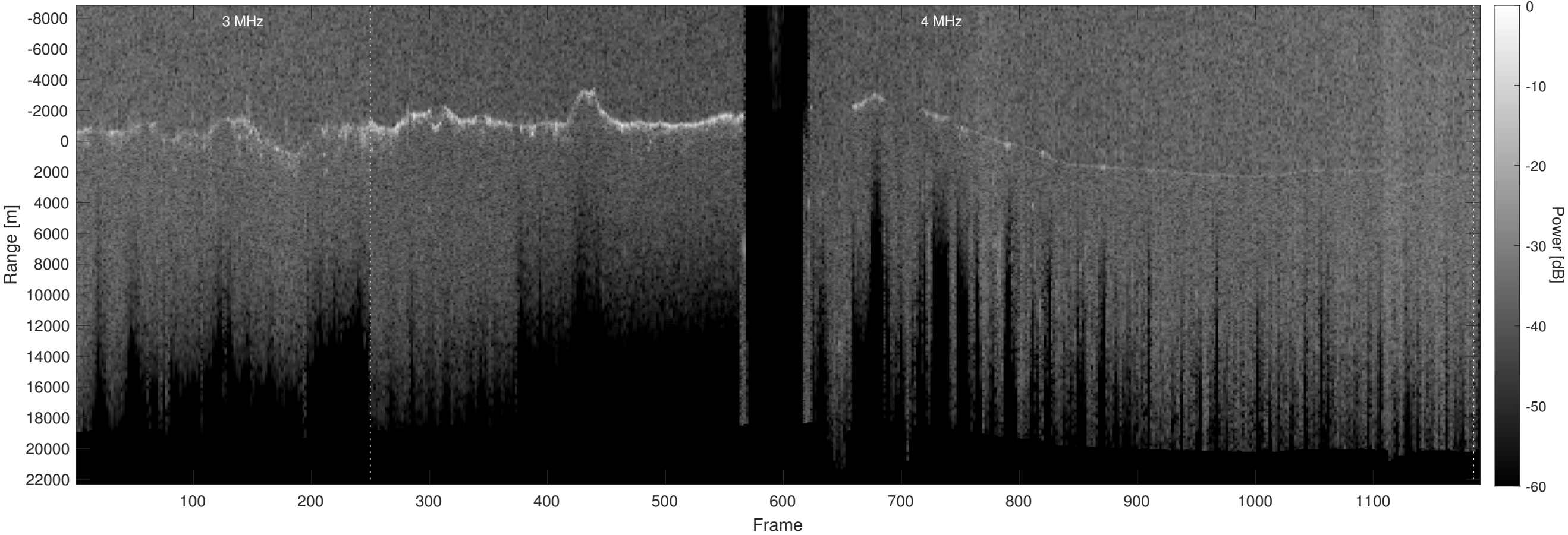
Orbit 12501, Optimized, Window, Depth-Corrected, Channel 2
