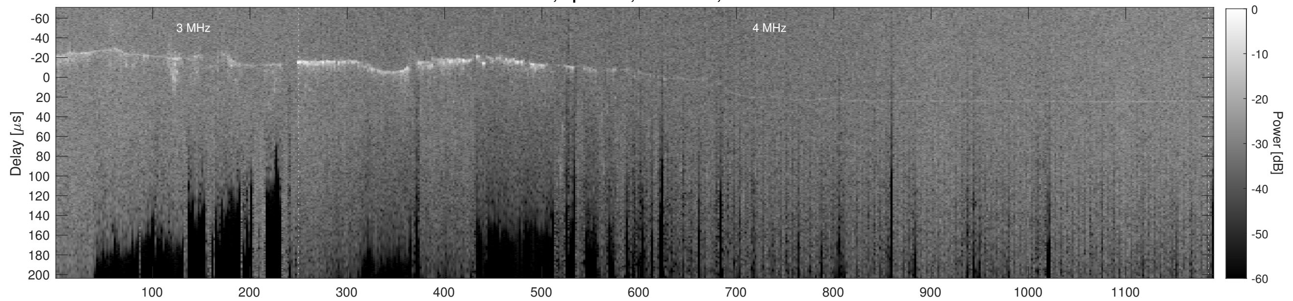
Orbit 12502, Cluttergram
