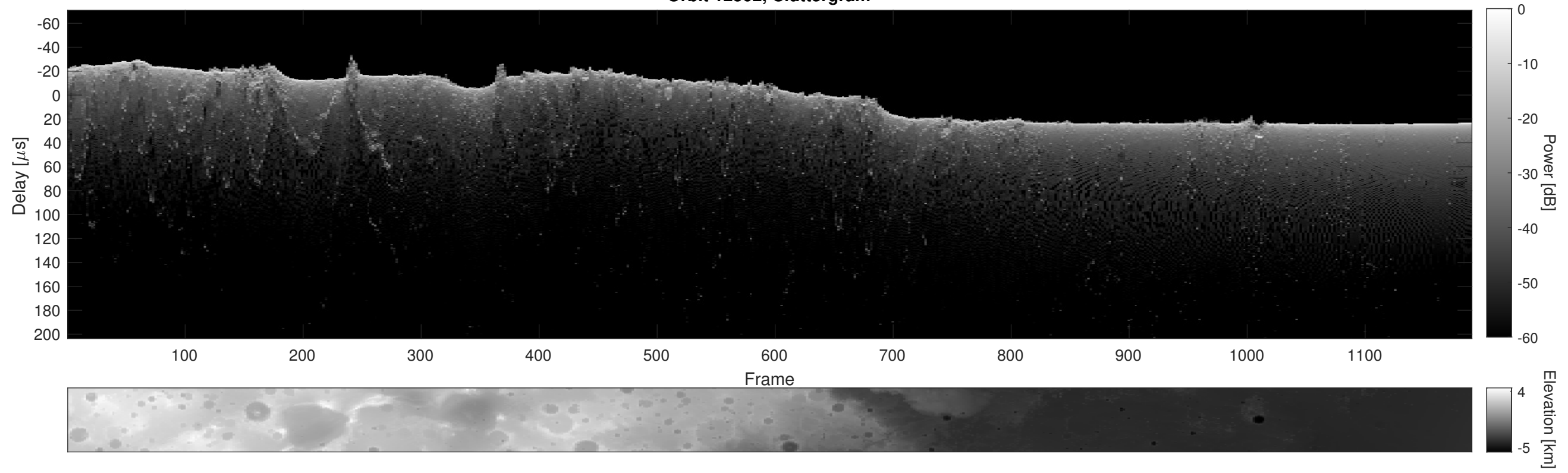
Orbit 12502, Cluttergram
