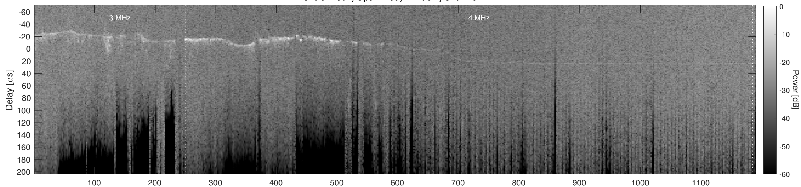
Orbit 12502, Cluttergram
