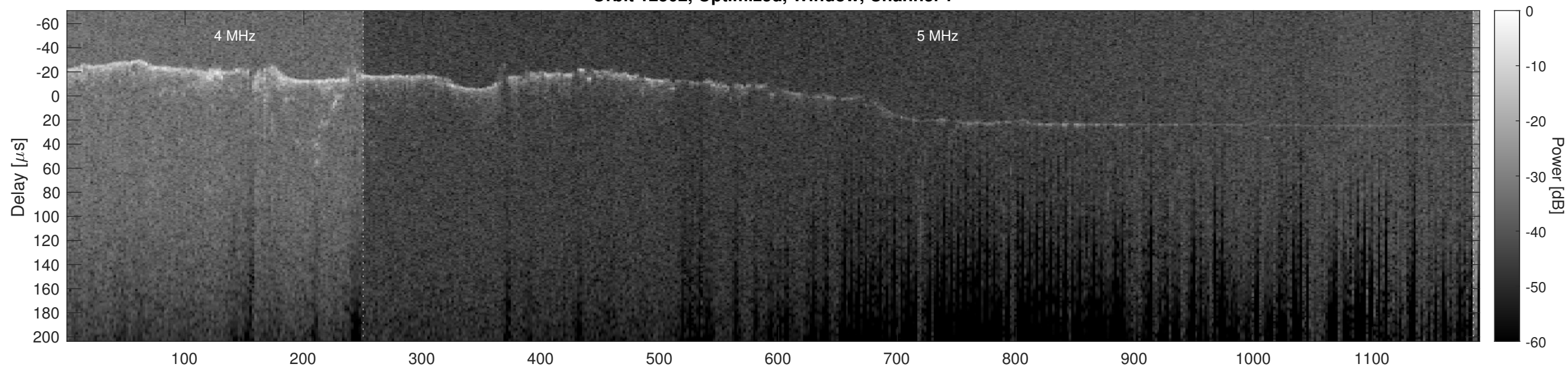
Orbit 12502, Optimized, Window, Channel 2
