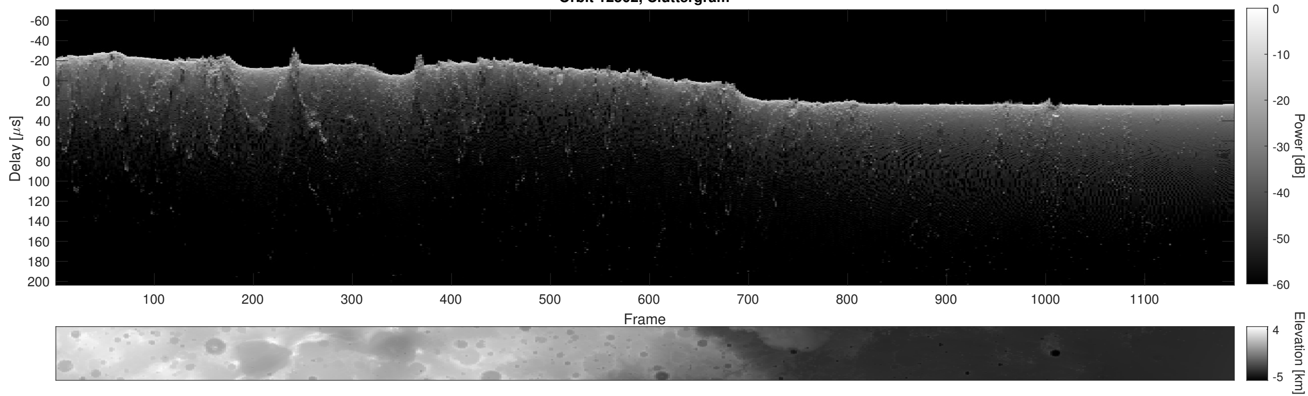
Orbit 12502, Cluttergram
