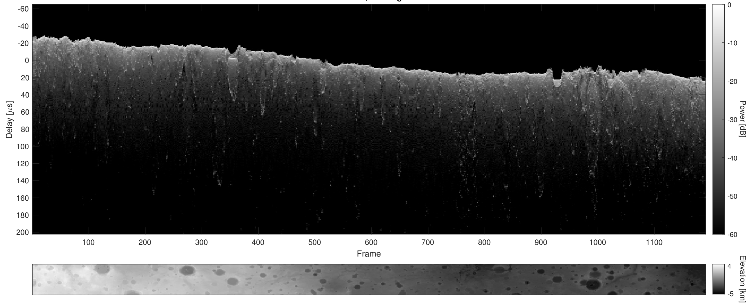
Orbit 12504, Cluttergram
