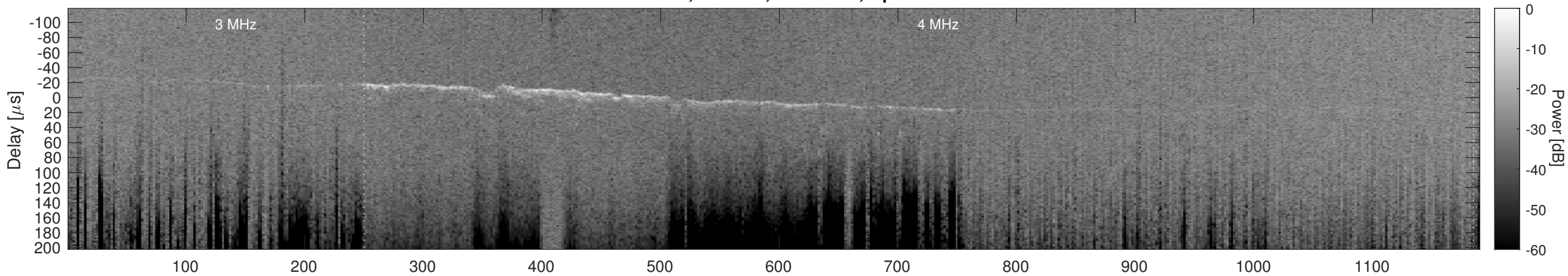
Orbit 12504, Cluttergram
