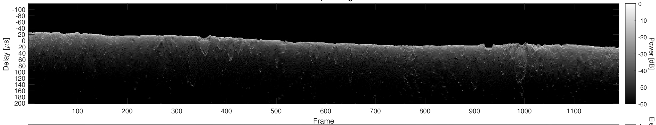
Orbit 12504, Cluttergram
