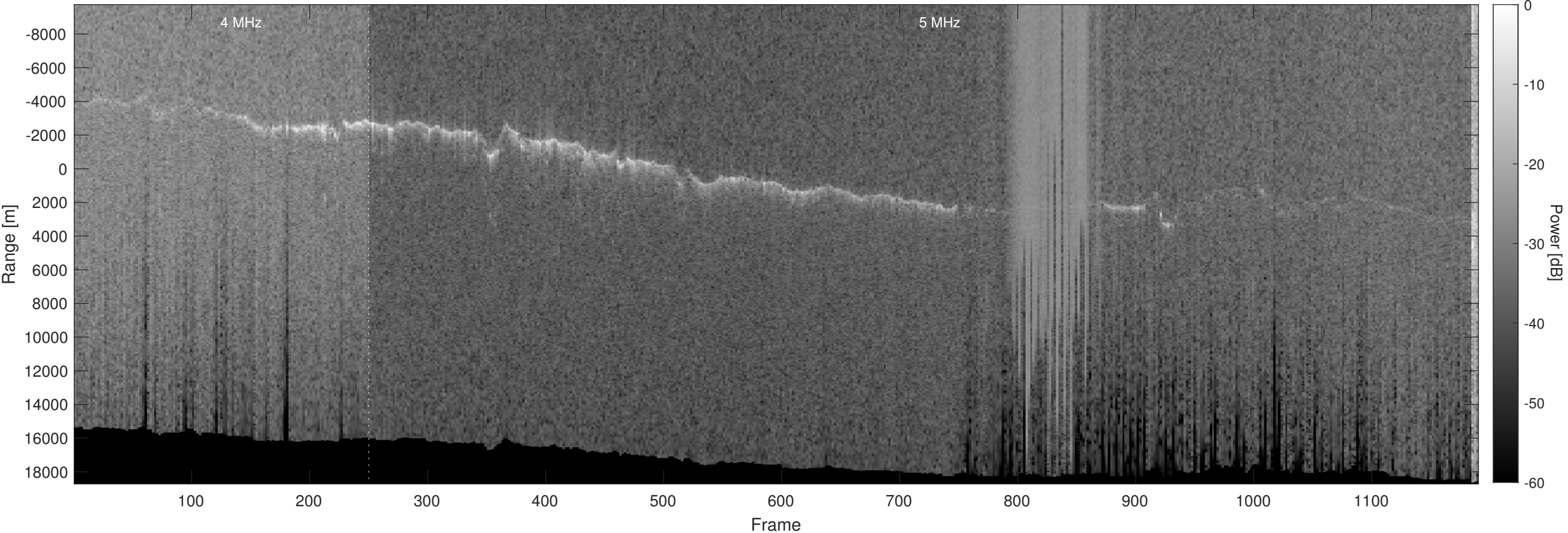
Orbit 12504, Optimized, No Window, Depth-Corrected, Channel 2
