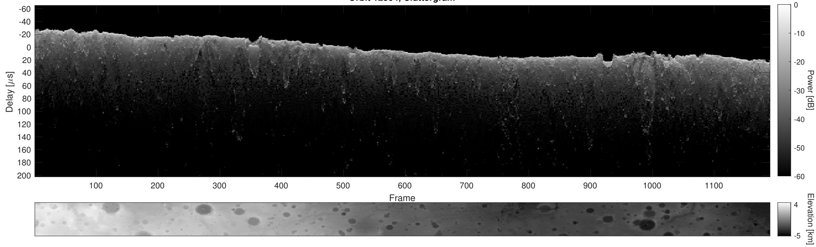
Orbit 12504, Cluttergram
