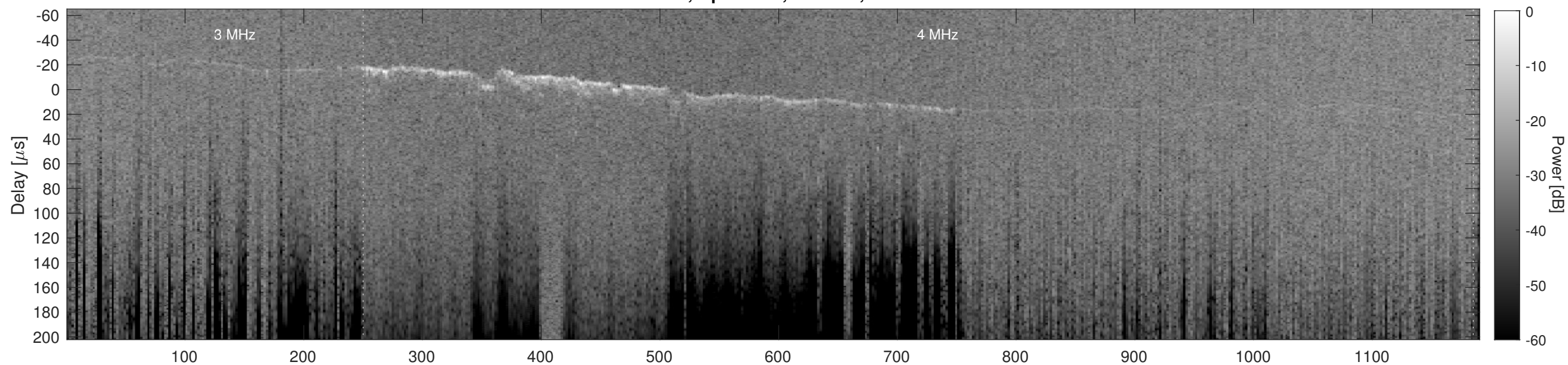
Orbit 12504, Cluttergram
