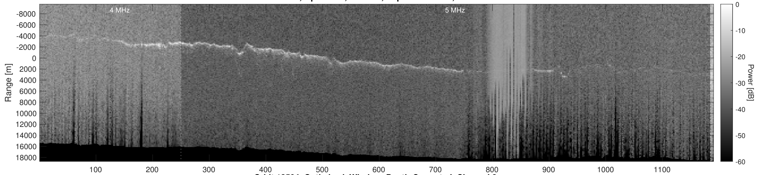
Orbit 12504, Optimized, Window, Depth-Corrected, Channel 2
