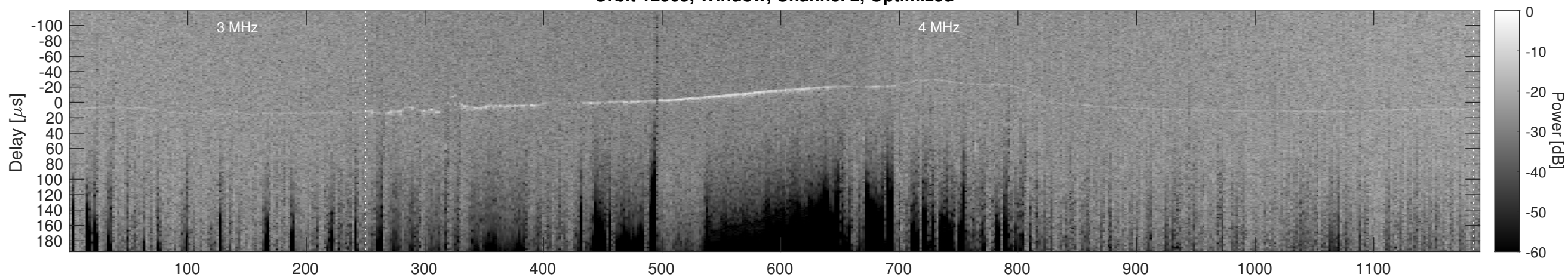
Orbit 12505, Cluttergram
