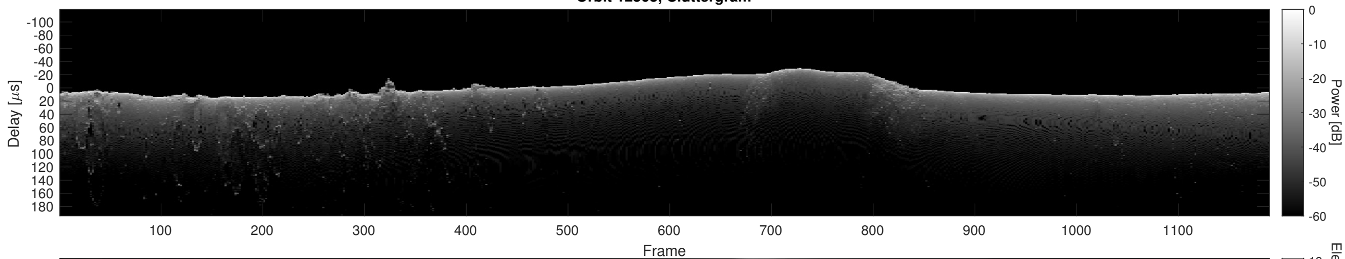
Orbit 12505, Cluttergram
