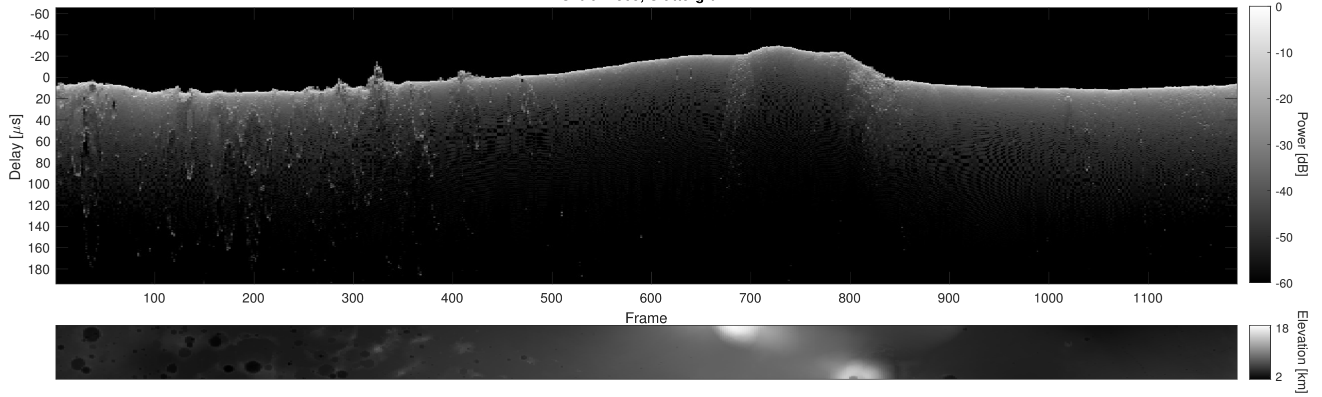
Orbit 12505, Cluttergram
