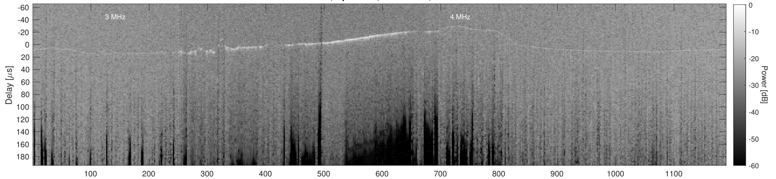
Orbit 12505, Cluttergram
