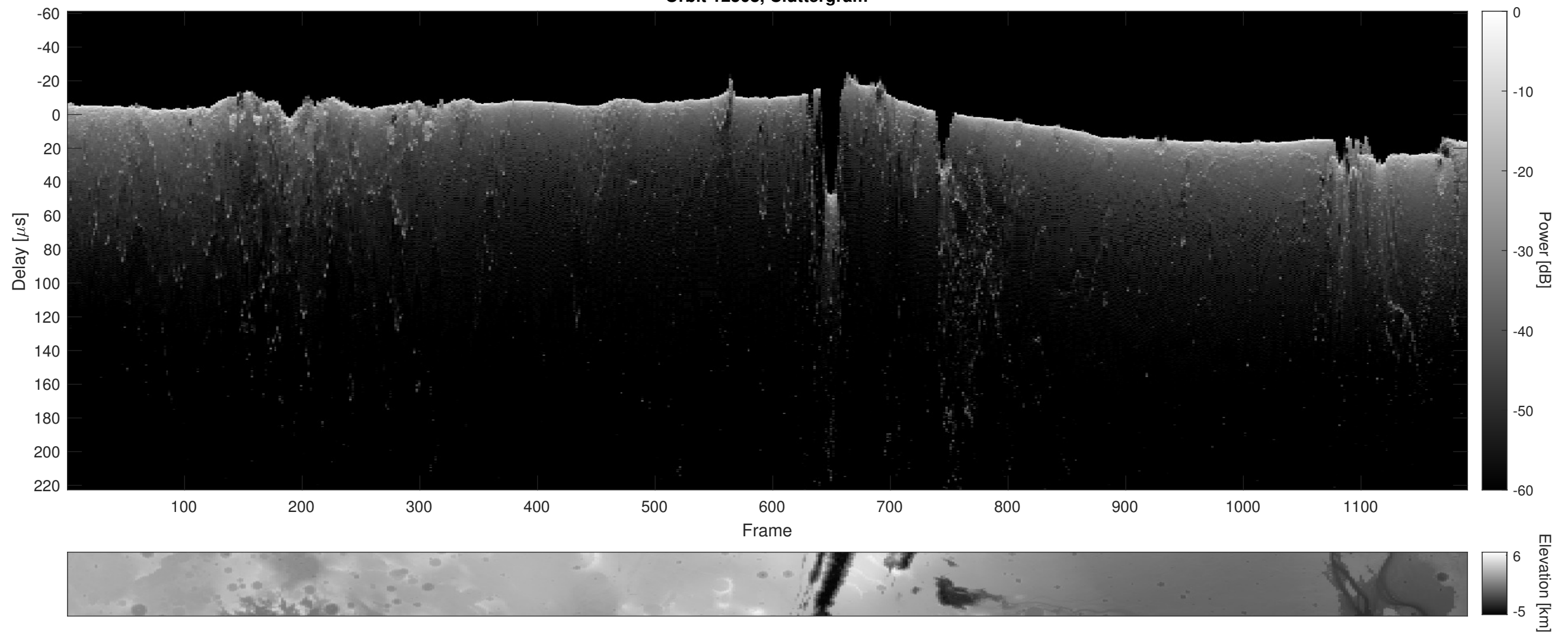
Orbit 12508, Cluttergram
