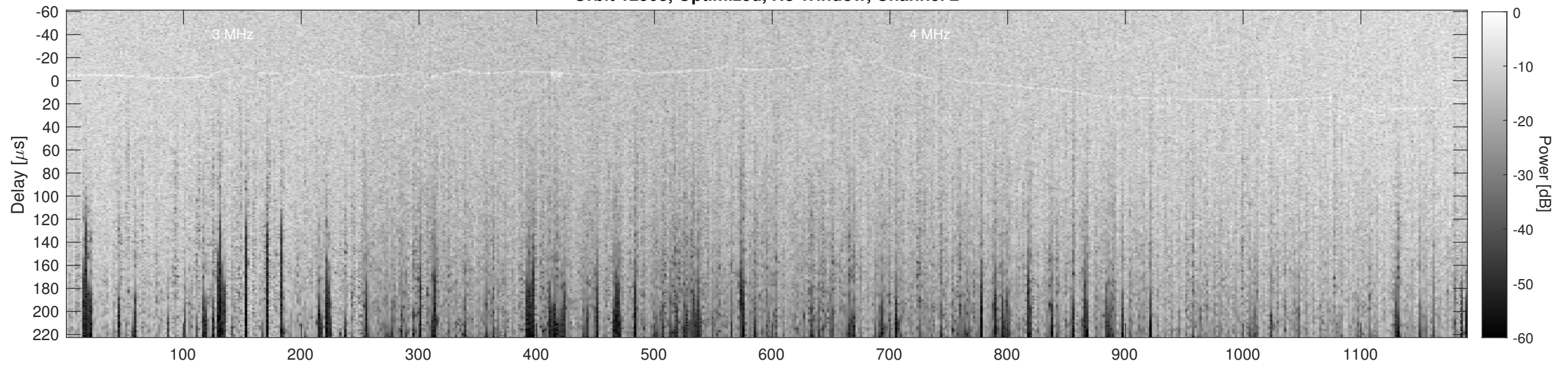
Orbit 12508, Cluttergram
