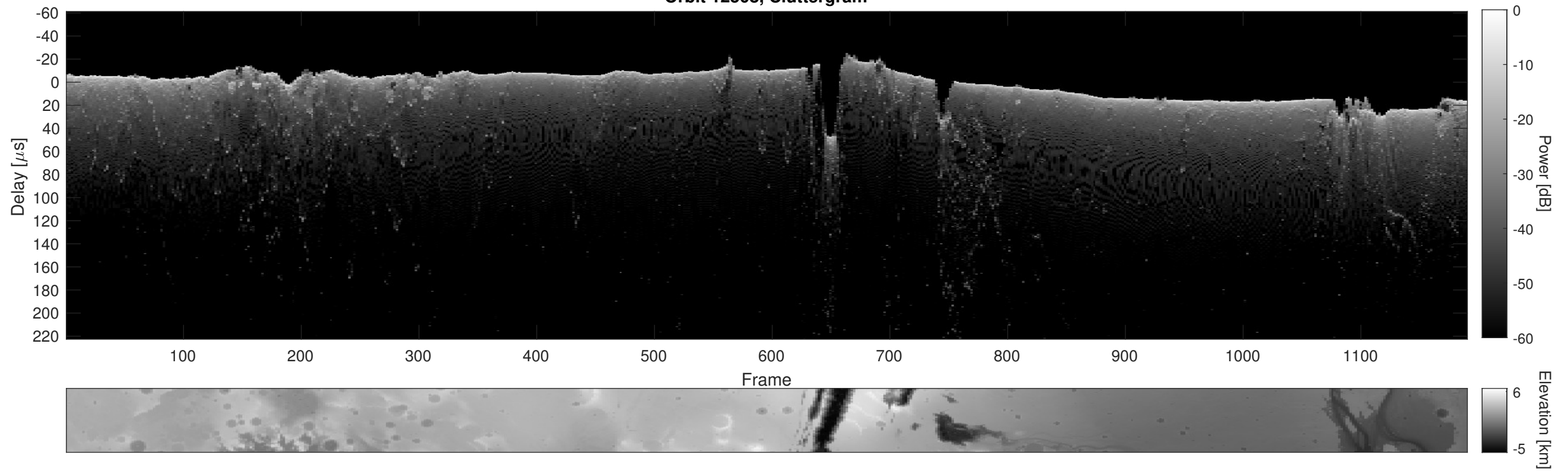
Orbit 12508, Cluttergram
