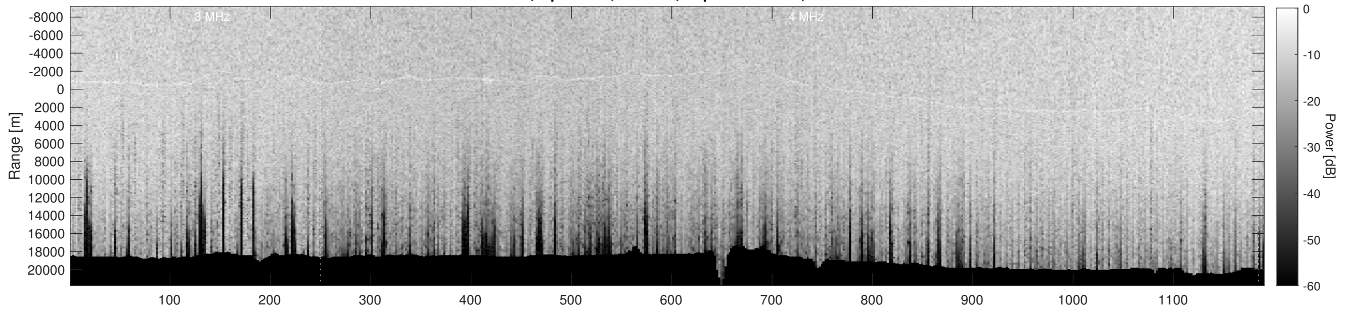
Orbit 12508, Depth-Corrected Cluttergram
