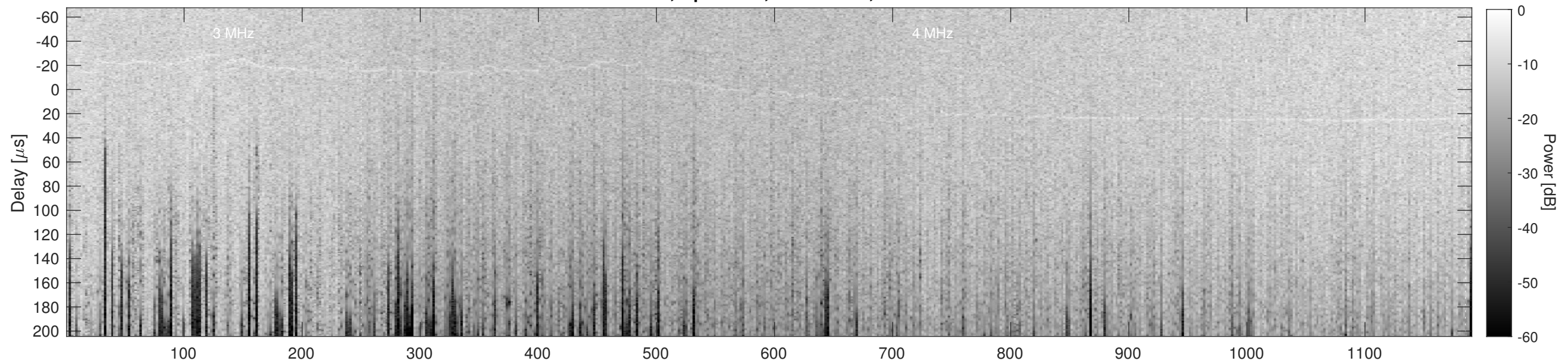
Orbit 12509, Cluttergram
