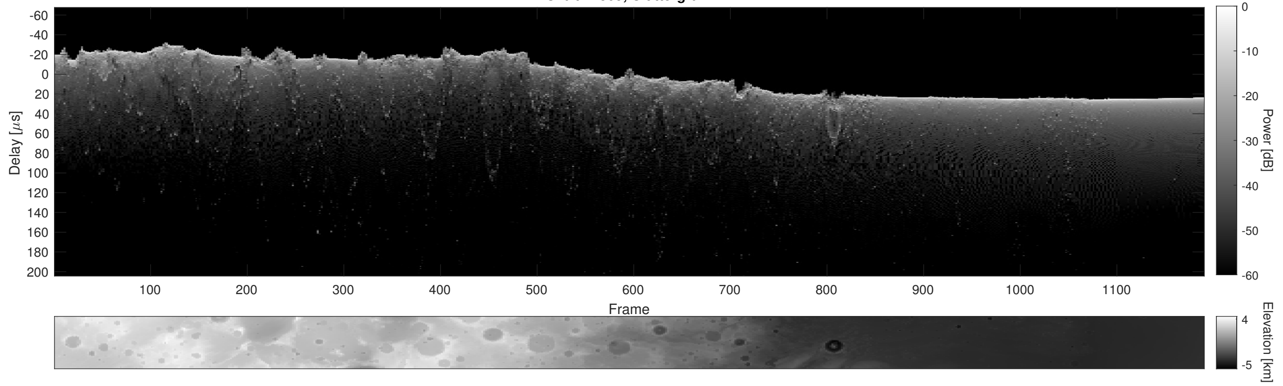
Orbit 12509, Cluttergram
