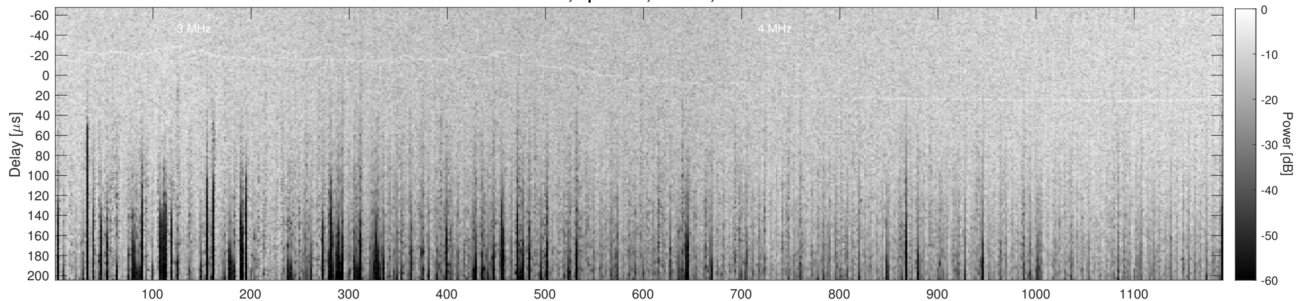
Orbit 12509, Cluttergram
