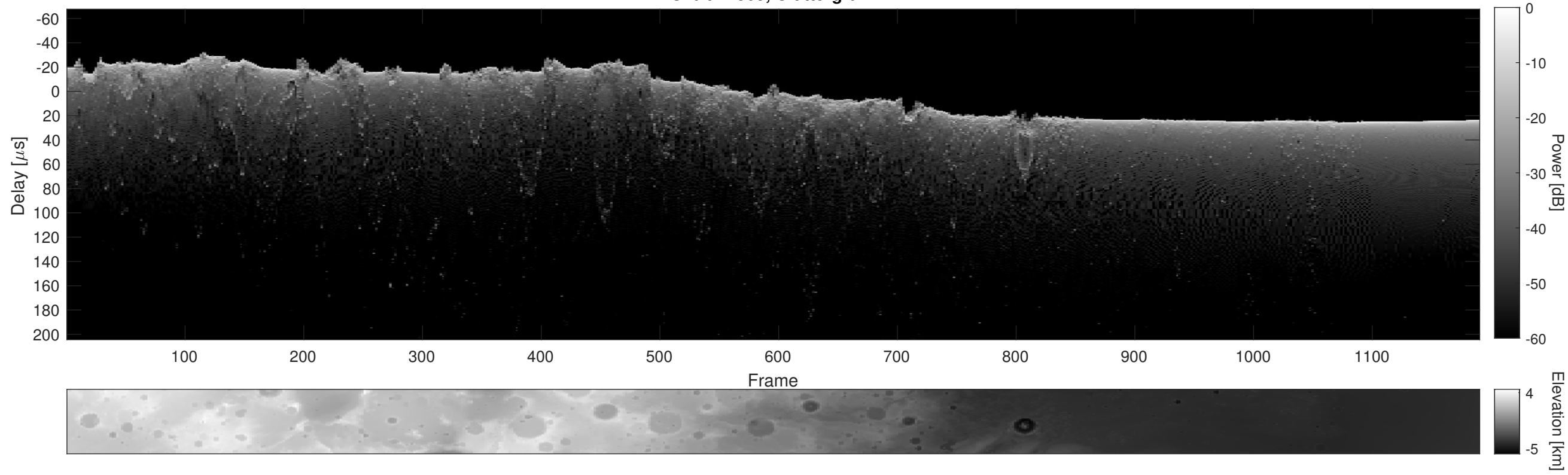
Orbit 12509, Cluttergram
