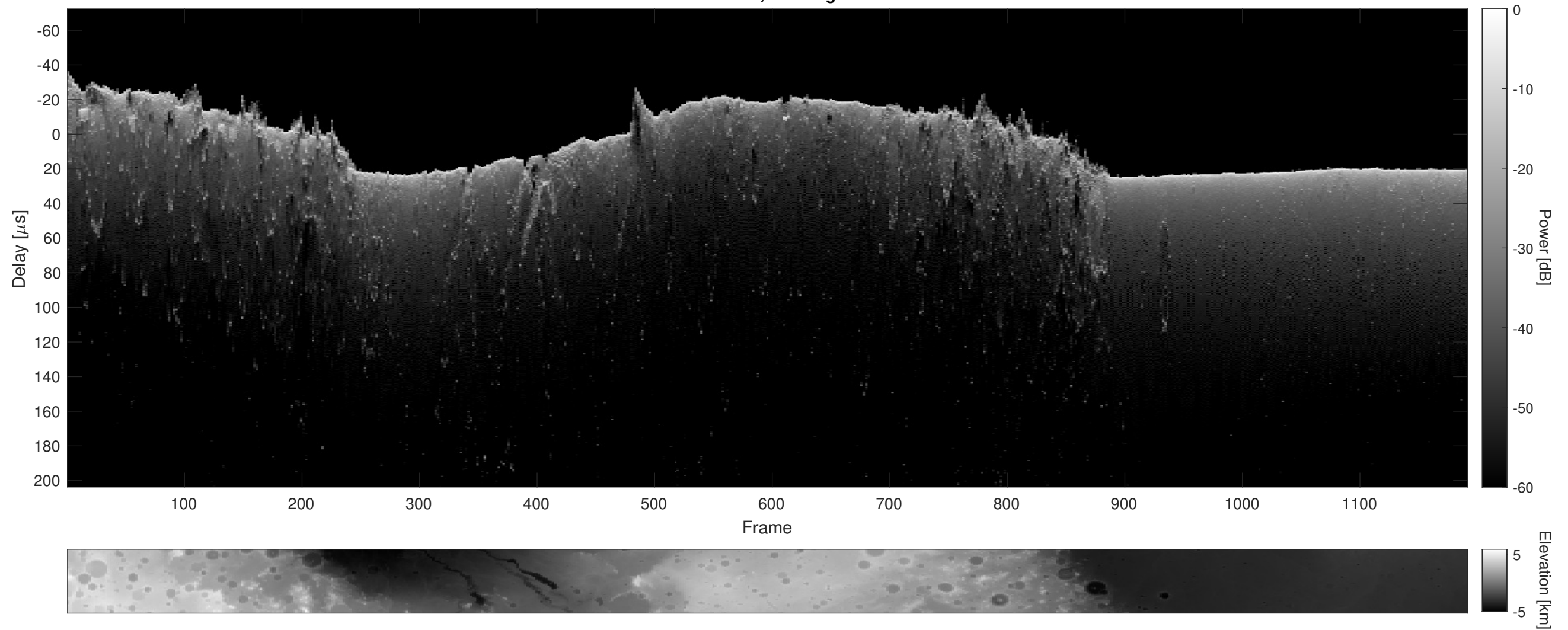
Orbit 12510, Cluttergram
