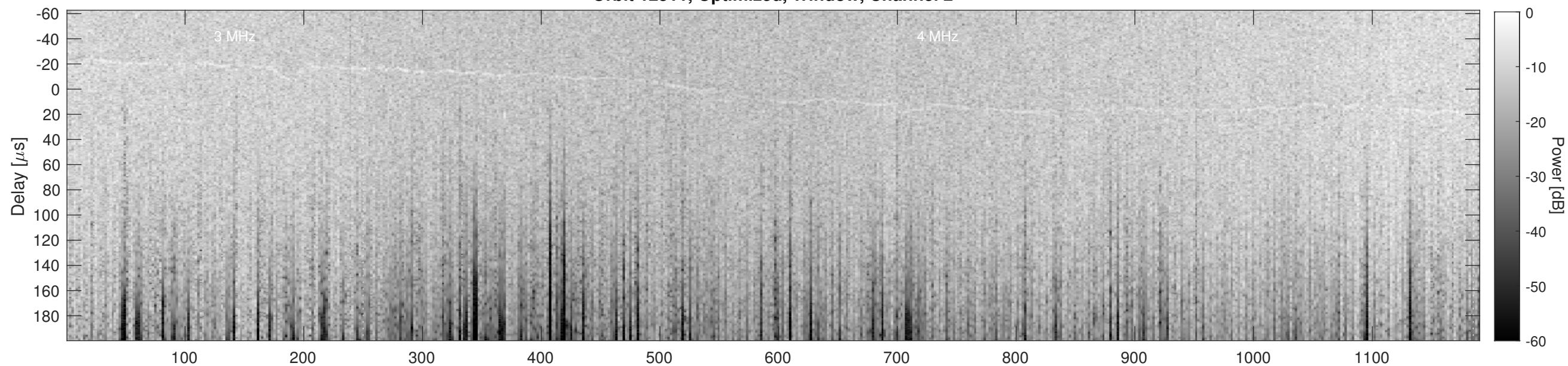
Orbit 12511, Cluttergram
