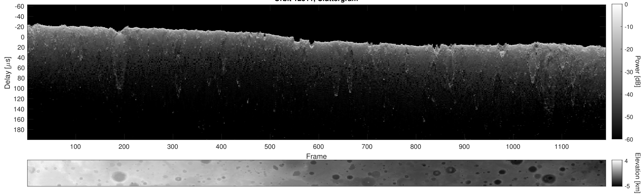
Orbit 12511, Cluttergram
