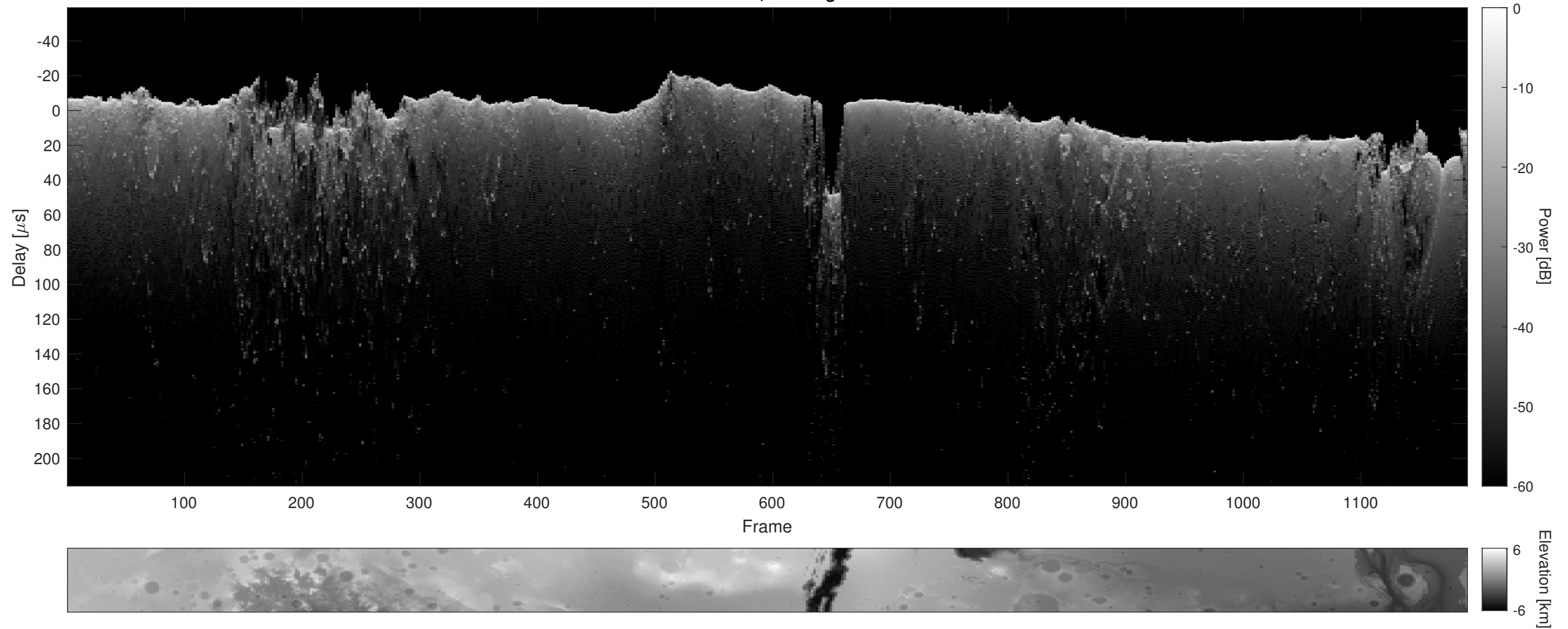
Orbit 12515, Cluttergram
