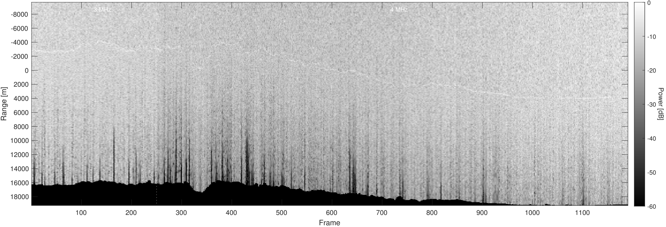
Orbit 12516, Optimized, No Window, Depth-Corrected, Channel 2
