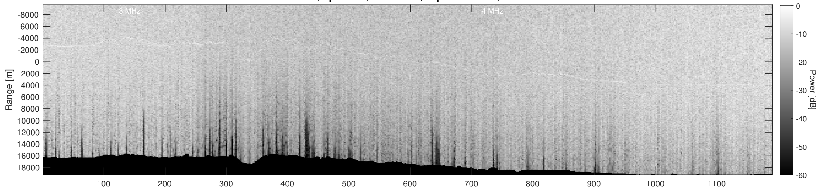
Orbit 12516, Depth-Corrected Cluttergram
