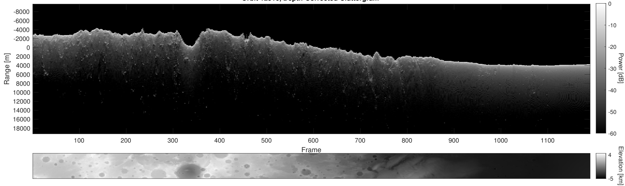
Orbit 12516, Depth-Corrected Cluttergram
