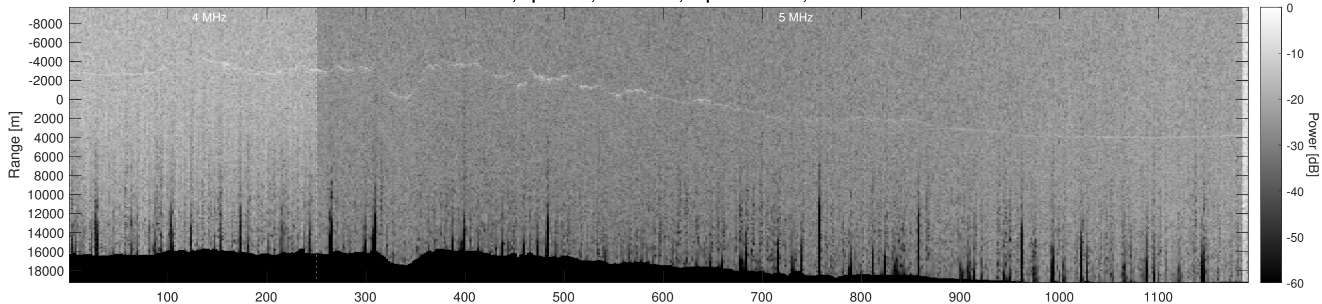
Orbit 12516, Optimized, No Window, Depth-Corrected, Channel 2
