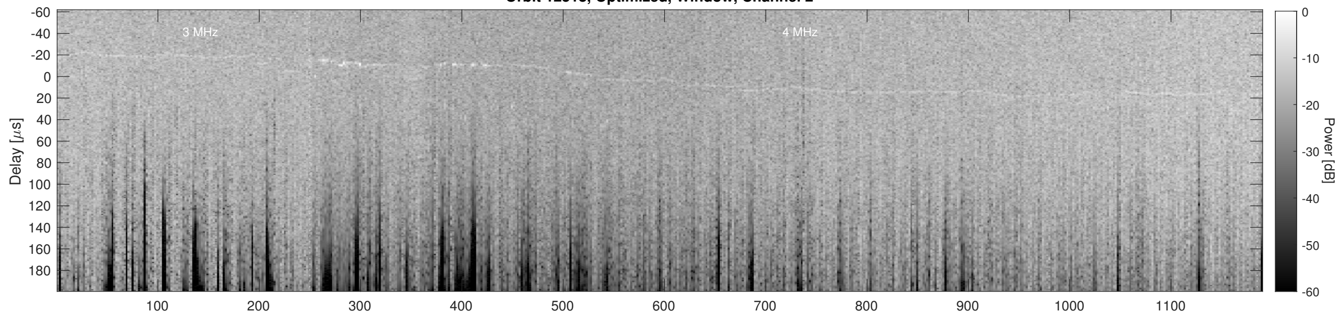
Orbit 12518, Cluttergram
