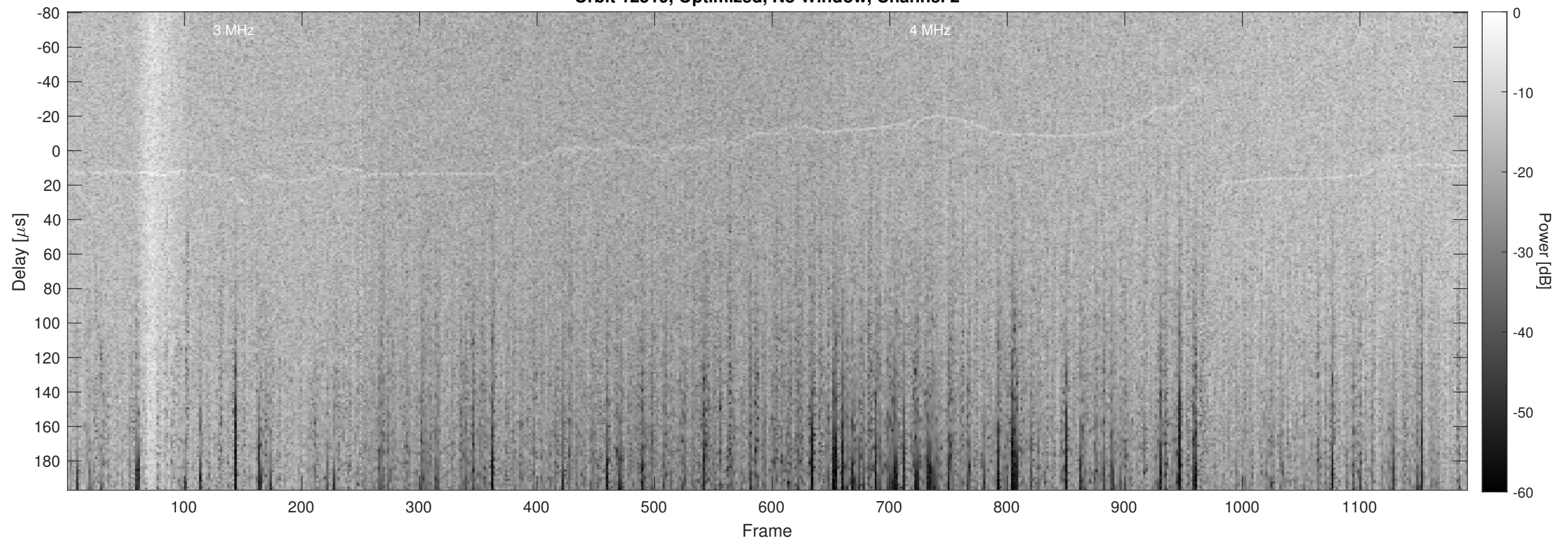
Orbit 12519, Optimized, No Window, Channel 2
