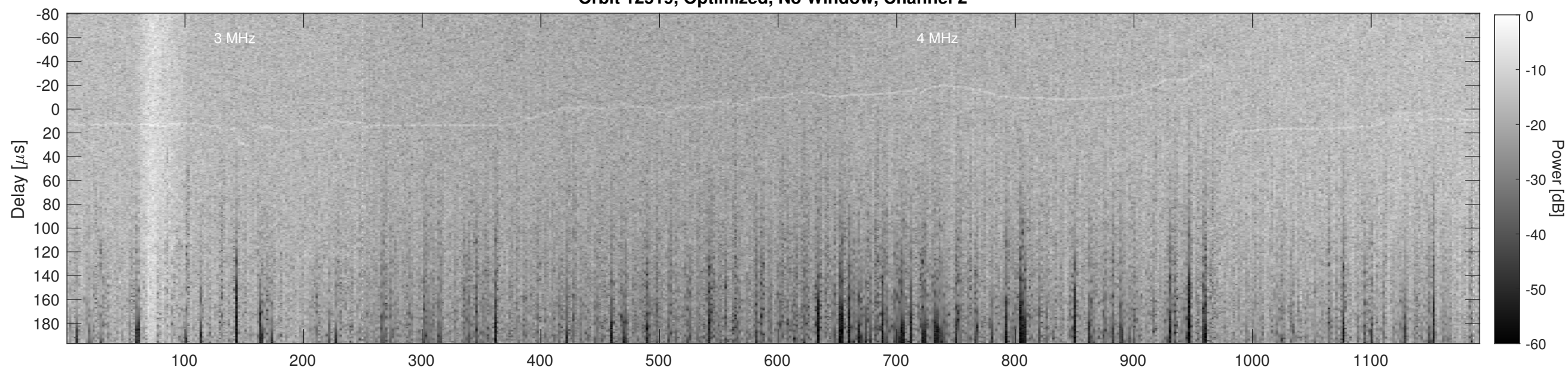
Orbit 12519, Cluttergram
