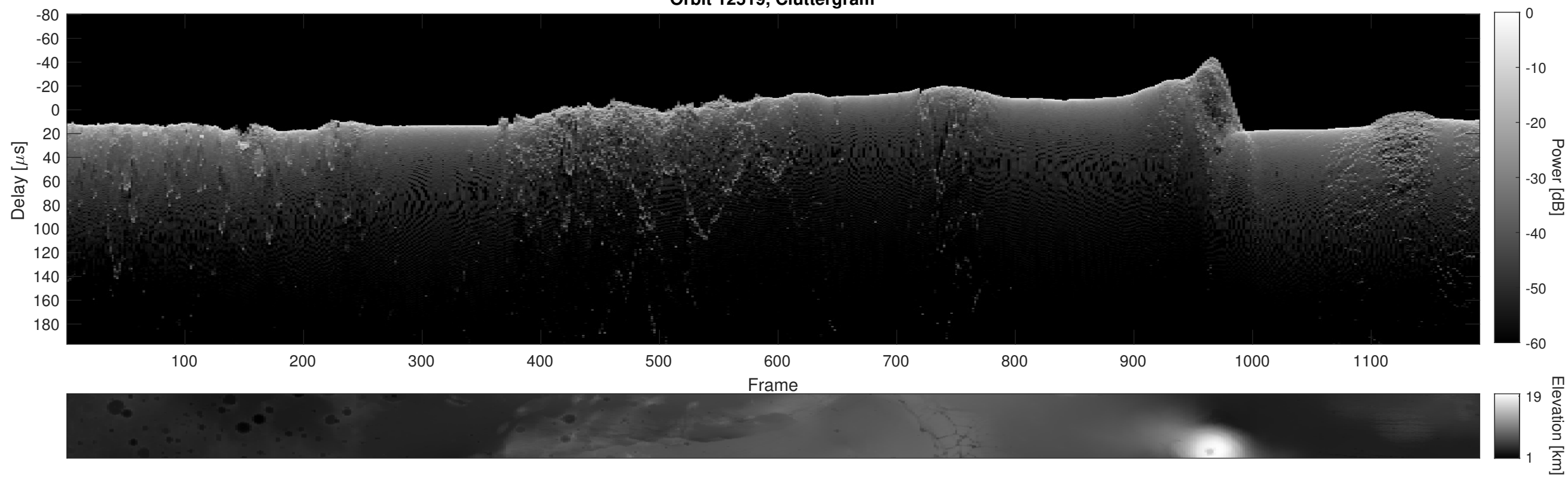
Orbit 12519, Cluttergram
