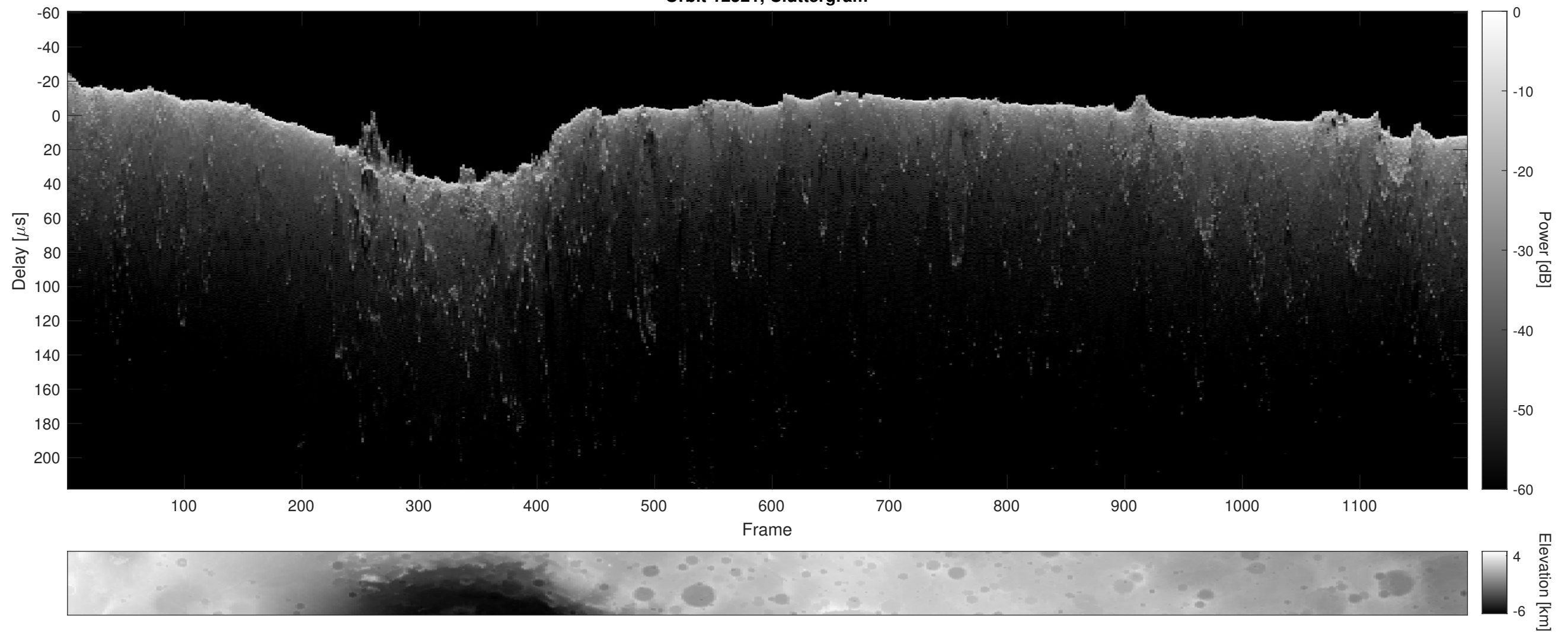
Orbit 12521, Cluttergram
