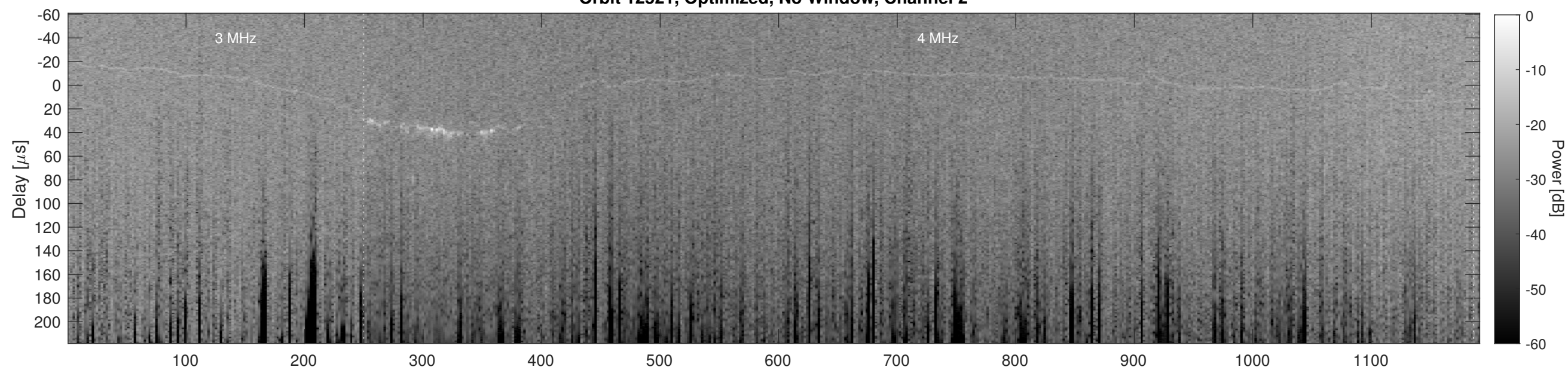
Orbit 12521, Cluttergram
