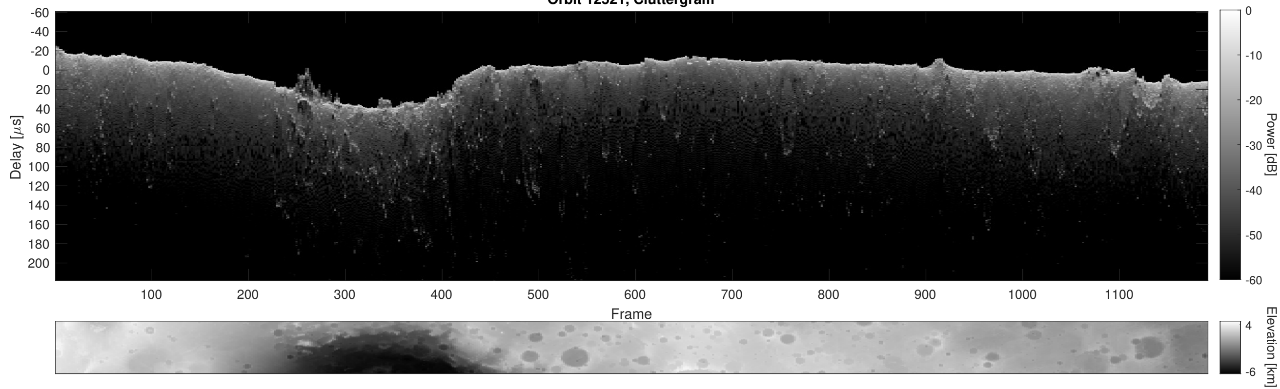
Orbit 12521, Cluttergram
