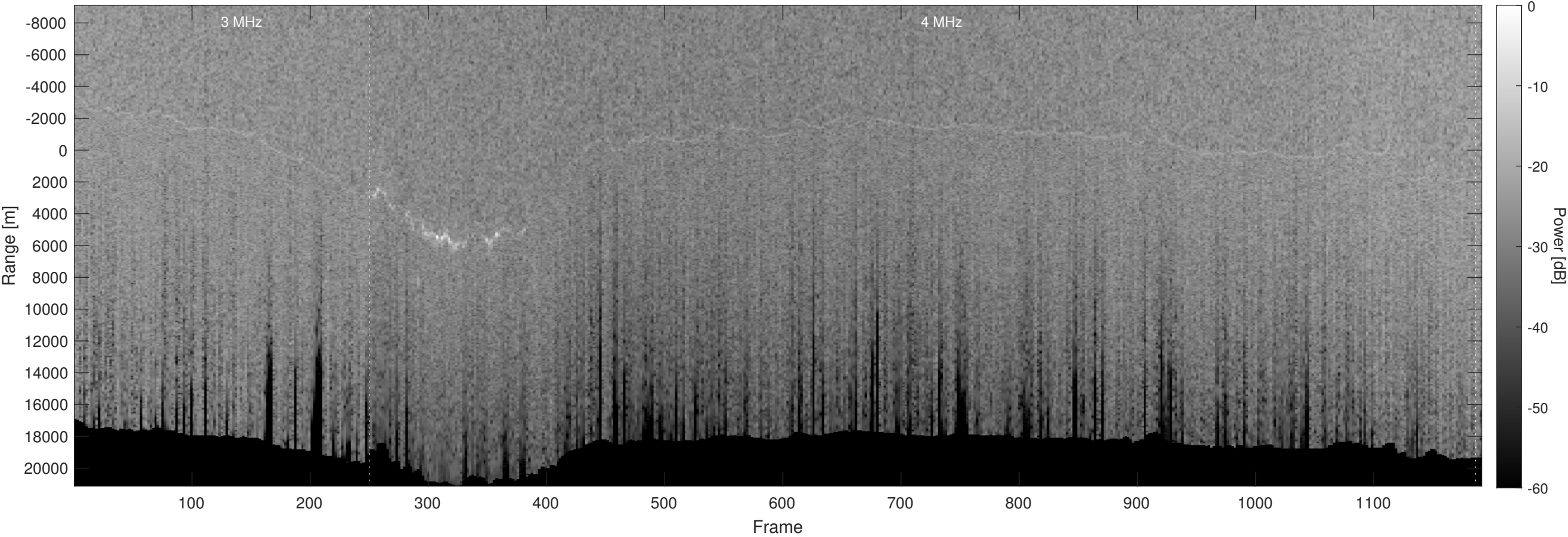
Orbit 12521, Optimized, No Window, Depth-Corrected, Channel 2
