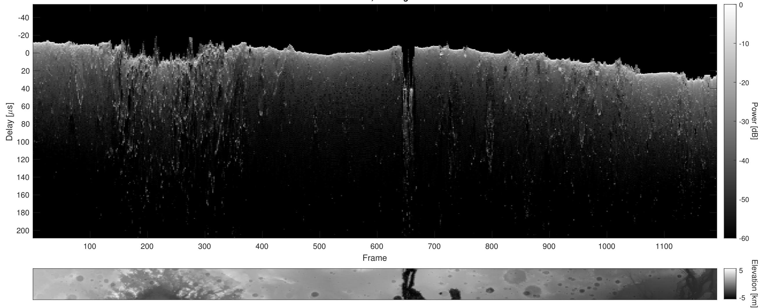
Orbit 12522, Cluttergram
