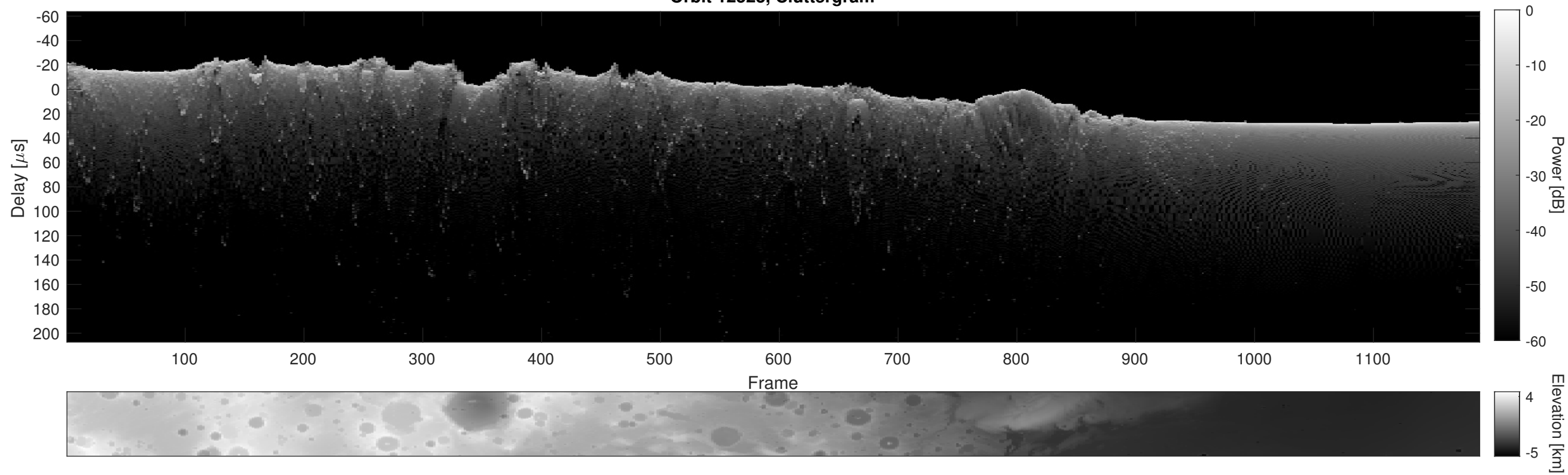
Orbit 12523, Cluttergram
