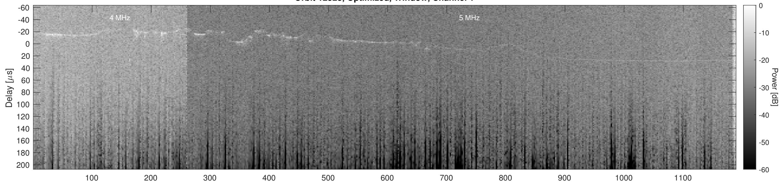
Orbit 12523, Optimized, Window, Channel 2
