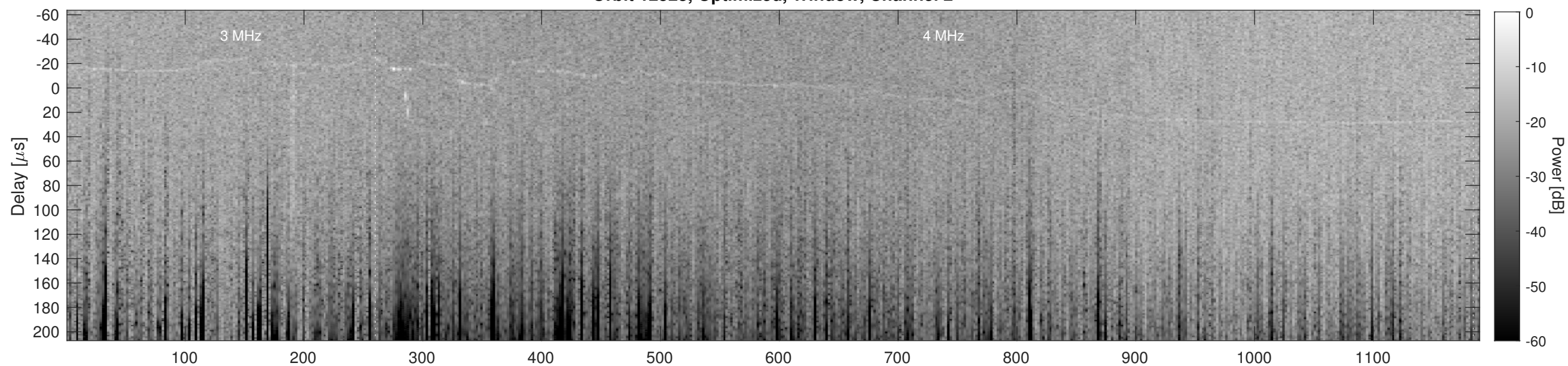
Orbit 12523, Cluttergram
