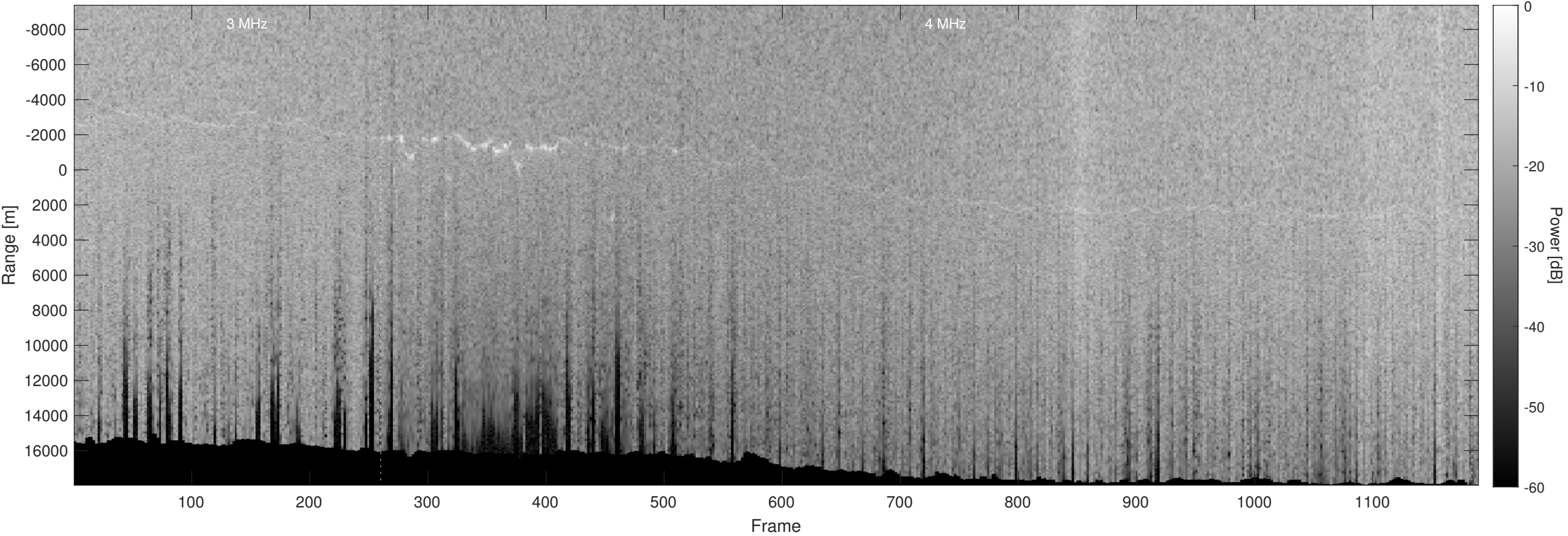
Orbit 12525, Optimized, No Window, Depth-Corrected, Channel 2
