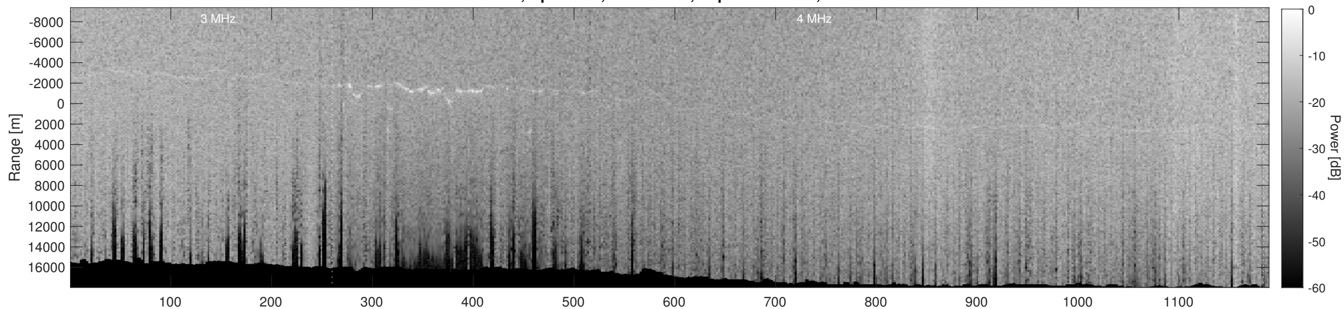
Orbit 12525, Depth-Corrected Cluttergram
