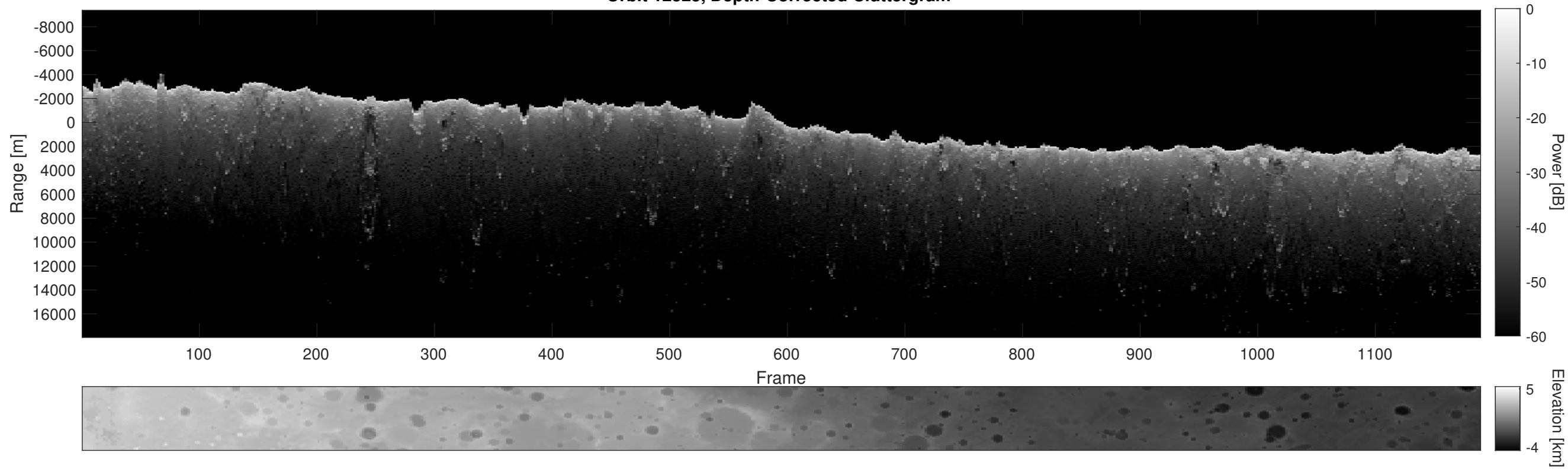
Orbit 12525, Depth-Corrected Cluttergram
