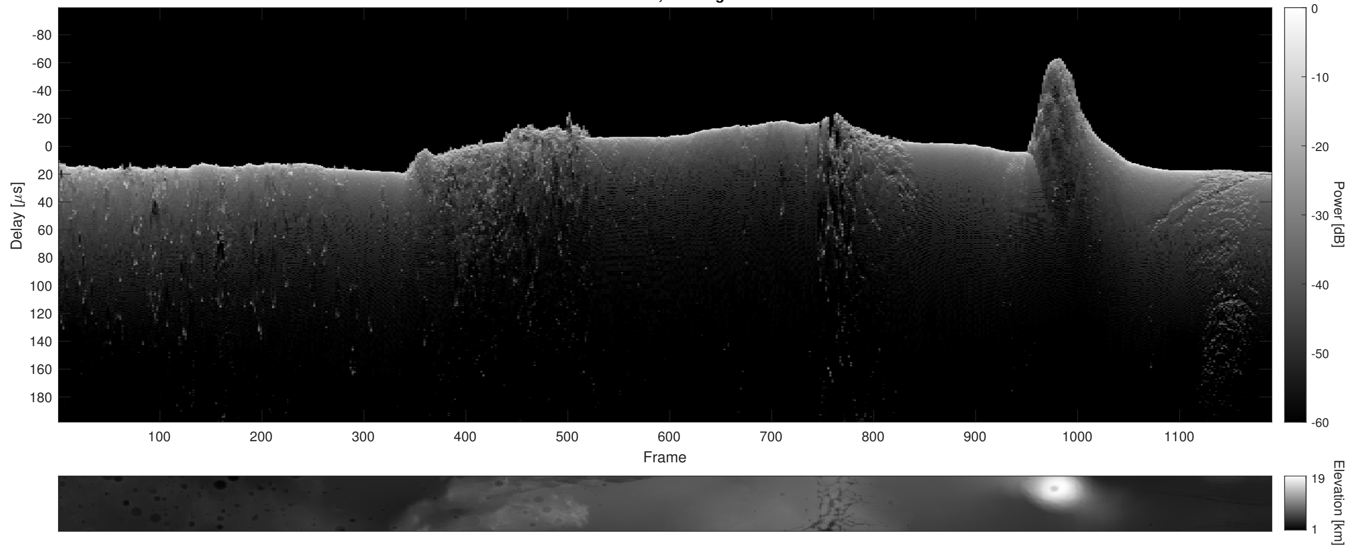
Orbit 12526, Cluttergram
