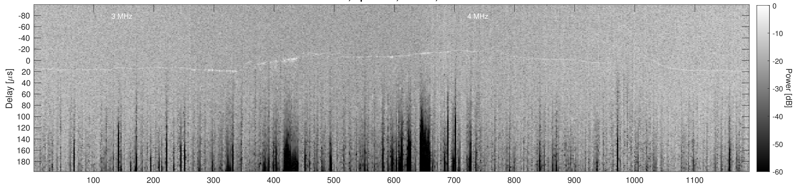
Orbit 12526, Cluttergram
