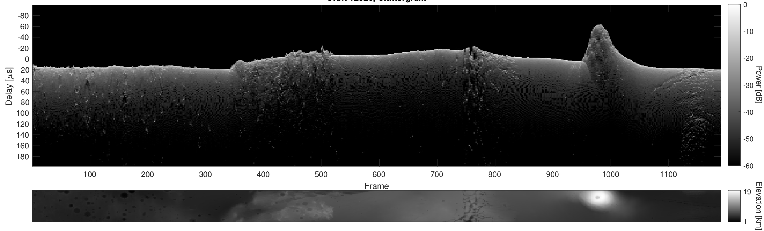
Orbit 12526, Cluttergram
