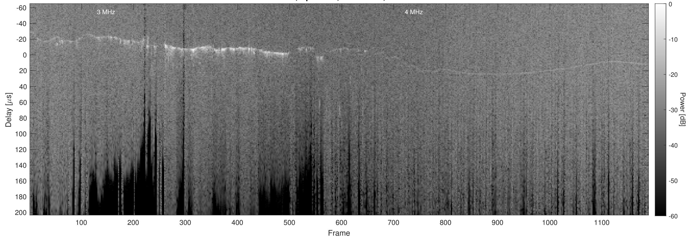
Orbit 12527, Optimized, No Window, Channel 2
