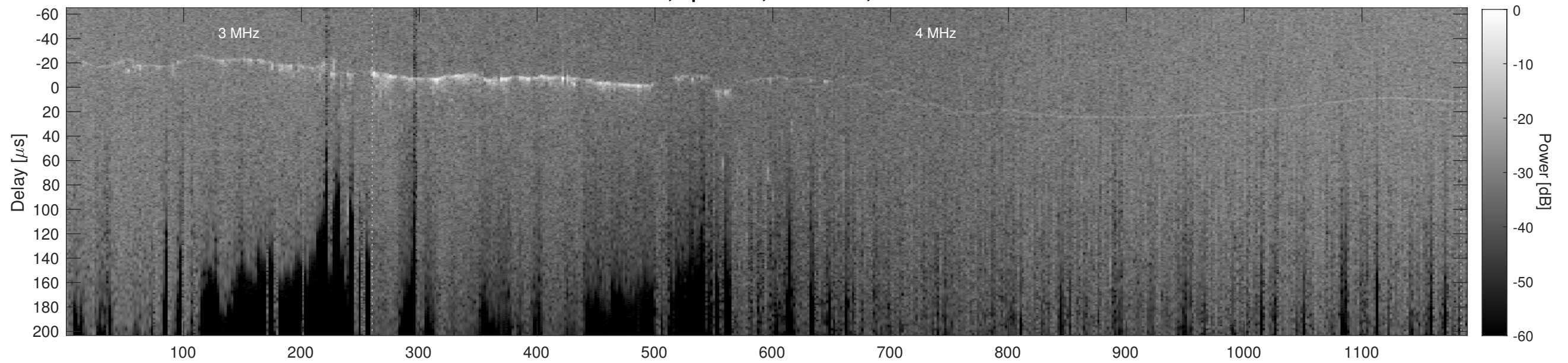
Orbit 12527, Cluttergram
