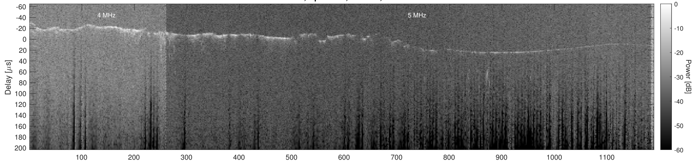
Orbit 12527, Optimized, Window, Channel 2
