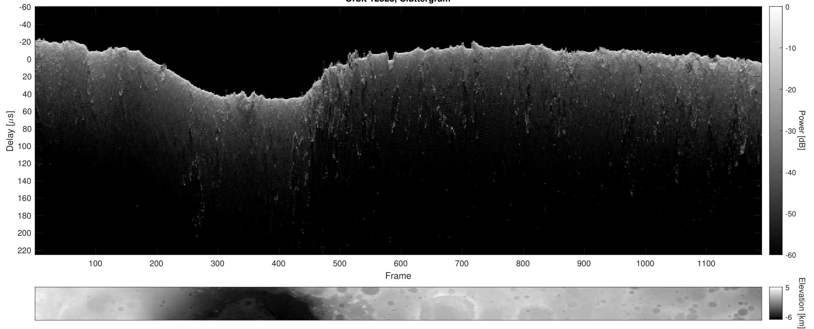
Orbit 12528, Cluttergram
