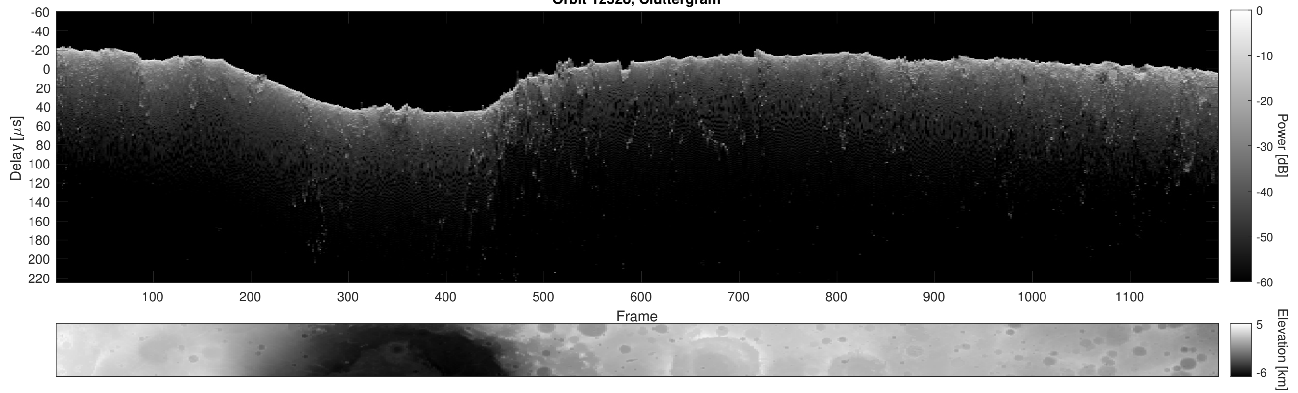
Orbit 12528, Cluttergram
