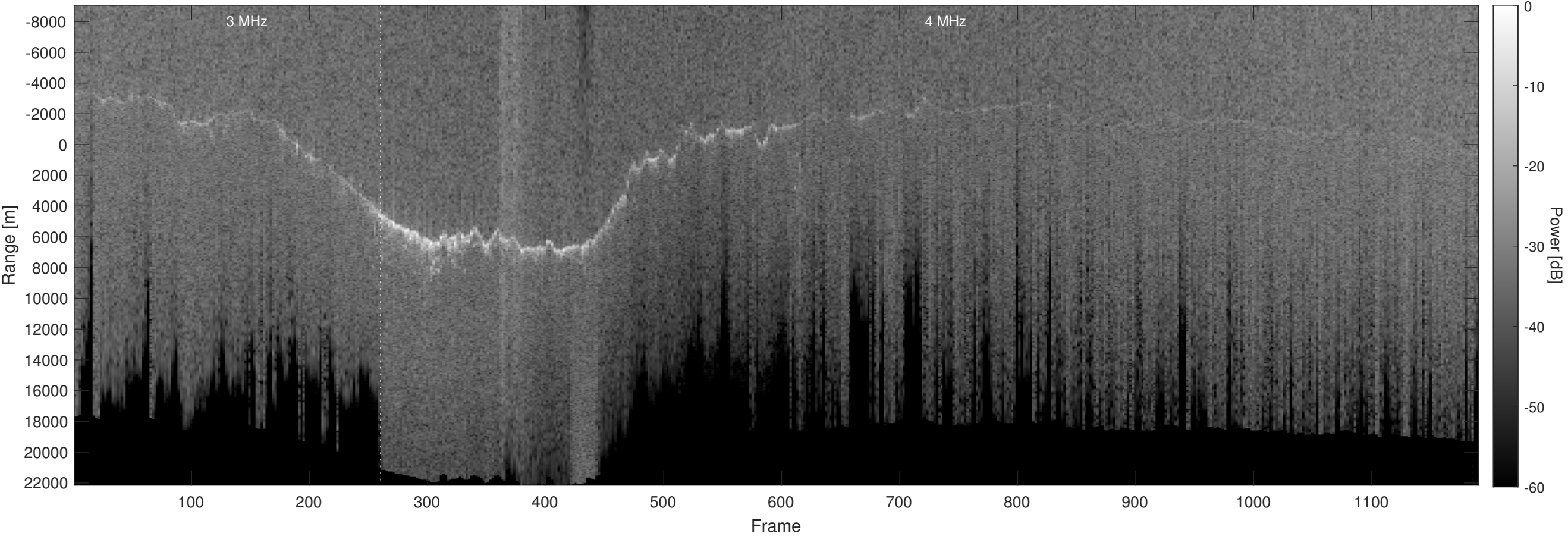
Orbit 12528, Optimized, No Window, Depth-Corrected, Channel 2
