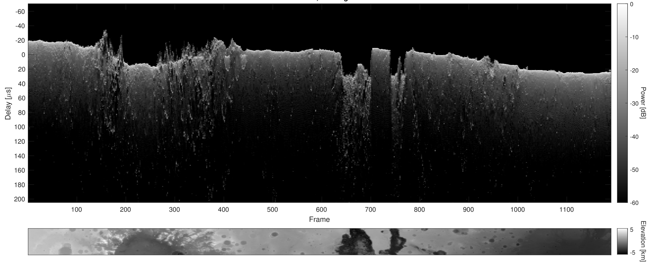
Orbit 12529, Cluttergram
