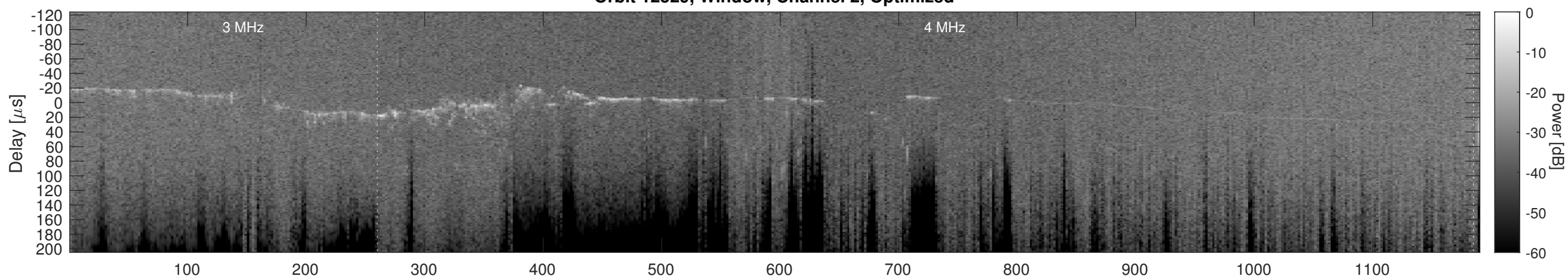
Orbit 12529, Cluttergram
