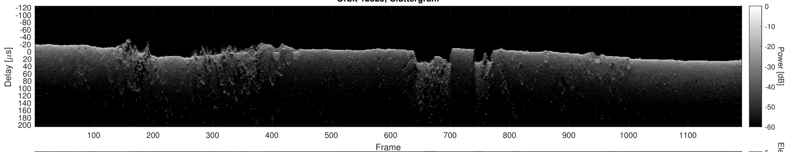
Orbit 12529, Cluttergram
