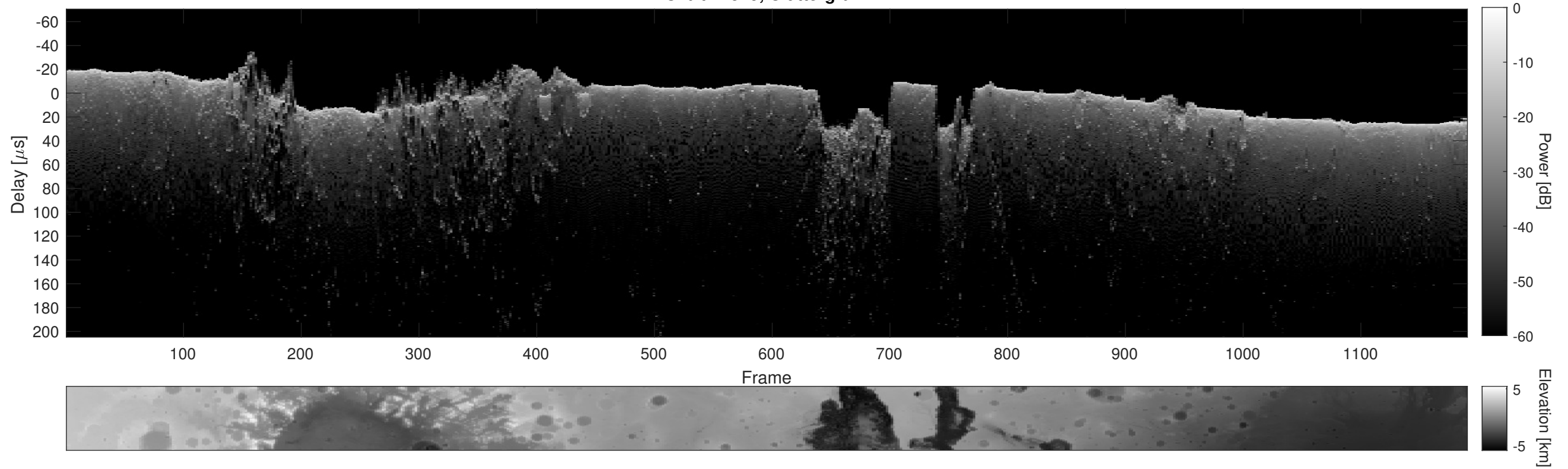
Orbit 12529, Cluttergram
