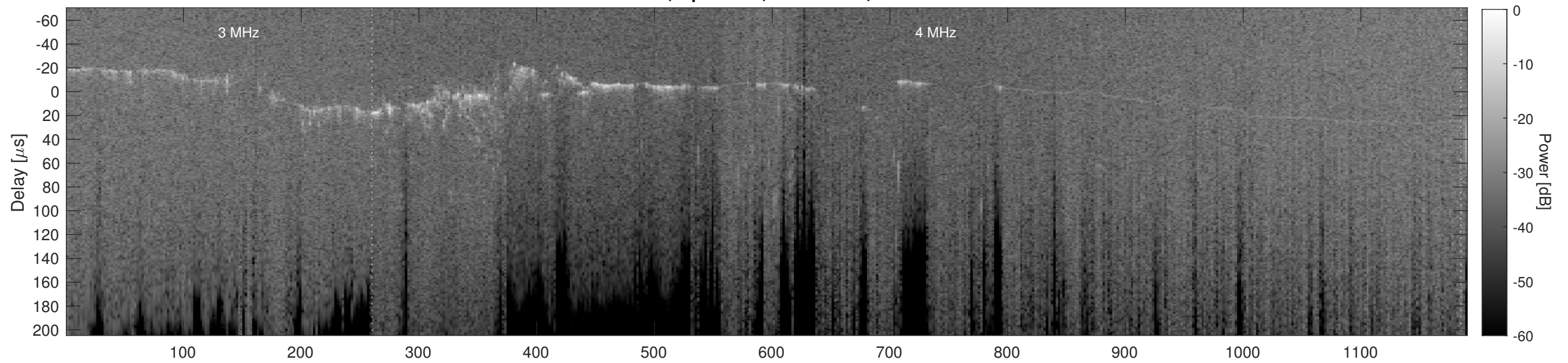
Orbit 12529, Cluttergram
