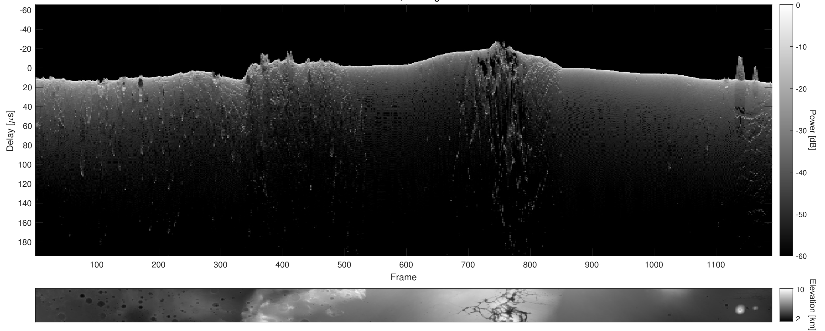
Orbit 12533, Cluttergram
