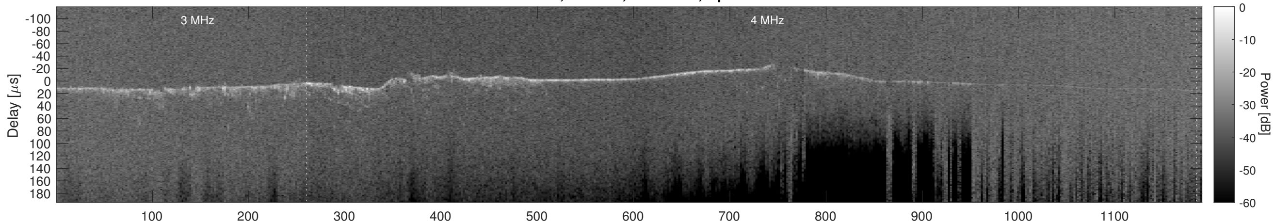
Orbit 12533, Cluttergram
