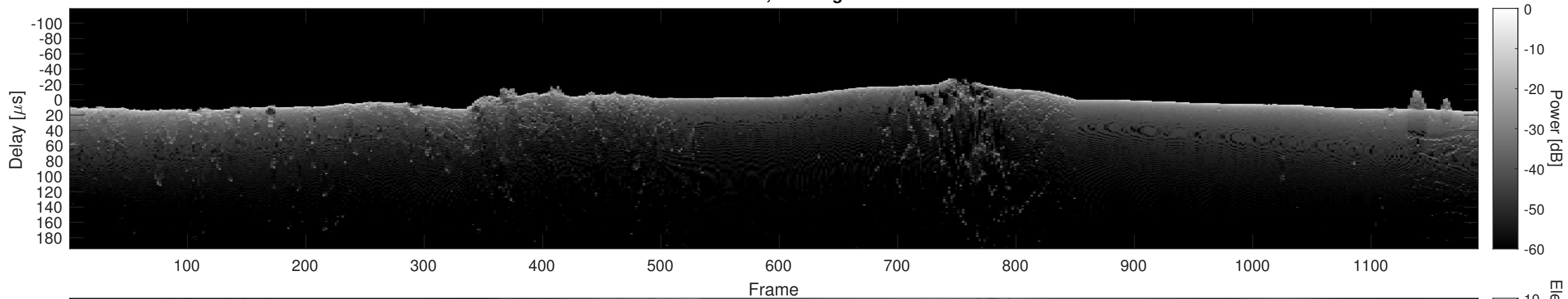
Orbit 12533, Cluttergram
