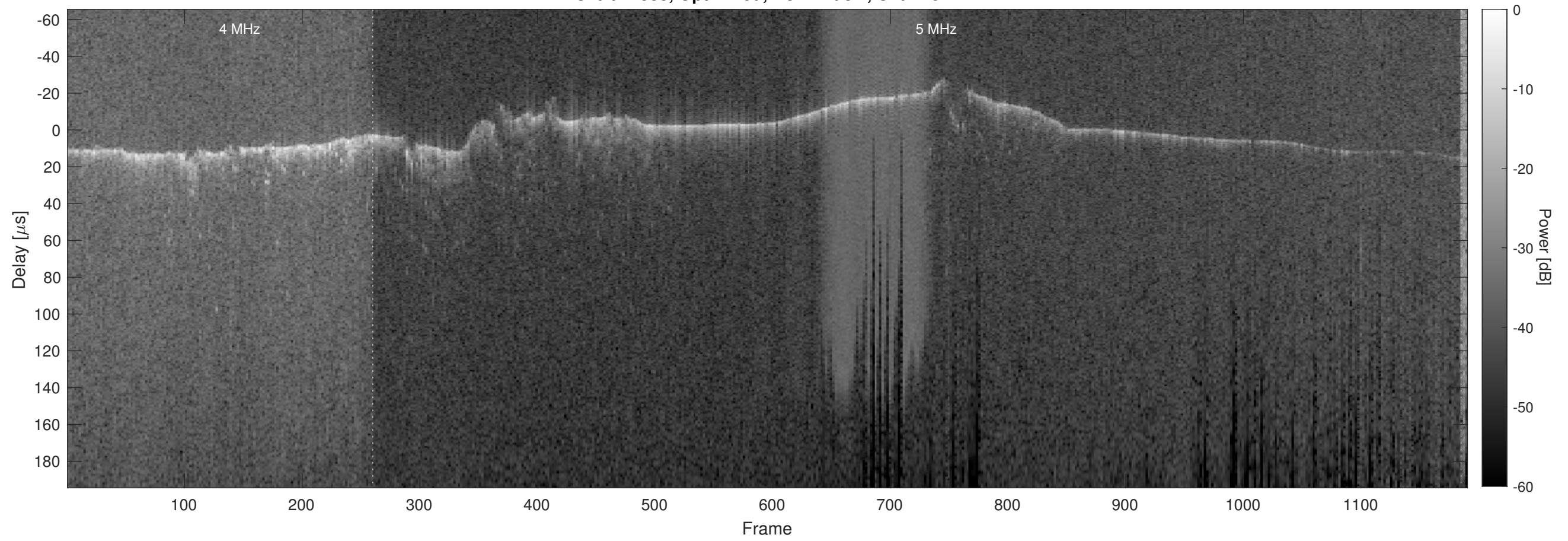
Orbit 12533, Optimized, No Window, Channel 2
