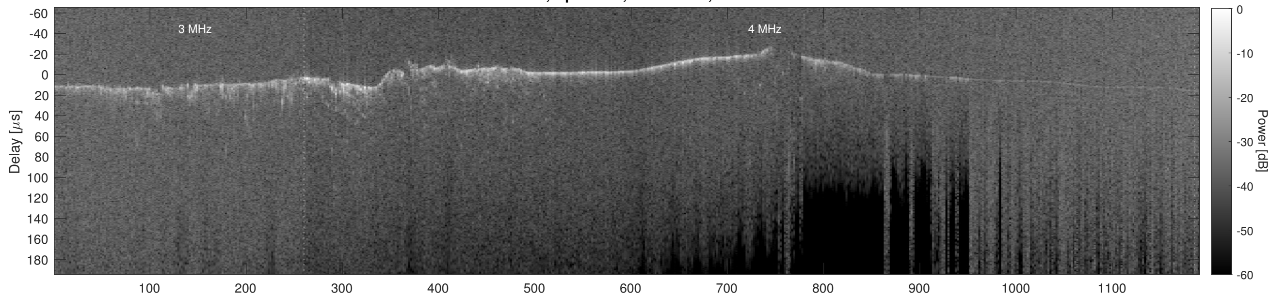
Orbit 12533, Cluttergram
